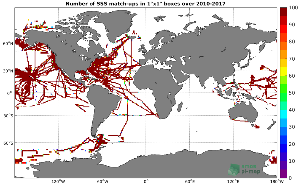
Figure 4: Number of SSS match-ups between TSG-SAMOS SSS and the SMOS-L4-CATDS-CECOS-IFREMER-V2-WEEKLY-0.5DEG SSS product for the Global Ocean Pi-MEP region over 1^\circ \times 1^\circ boxes and for the full satellite product period.
