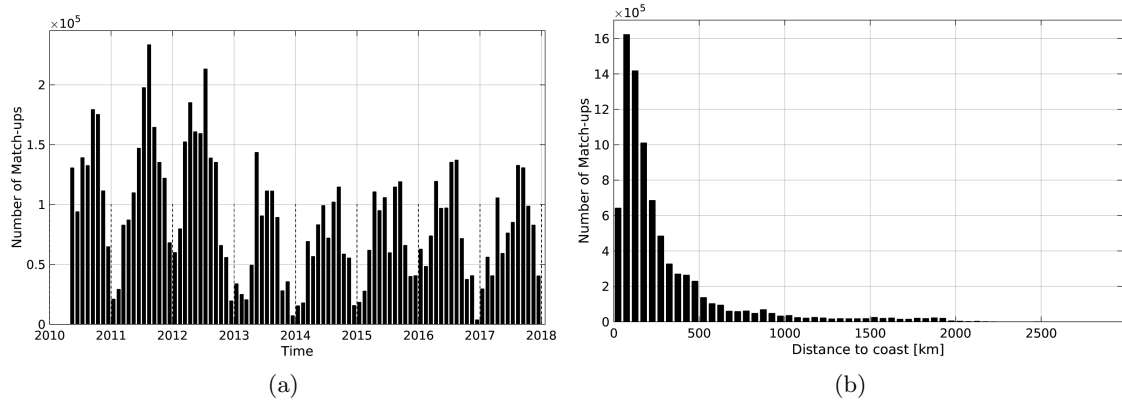
Figure 1: Number of match-ups between TSG-SAMOS and SMOS-L4-CATDS-CECOS-IFREMER-V2-WEEKLY-0.5DEG SSS as a function of time (a) and as function of the distance to coast (b) over the Global Ocean Pi-MEP region and for the full satellite product period.
