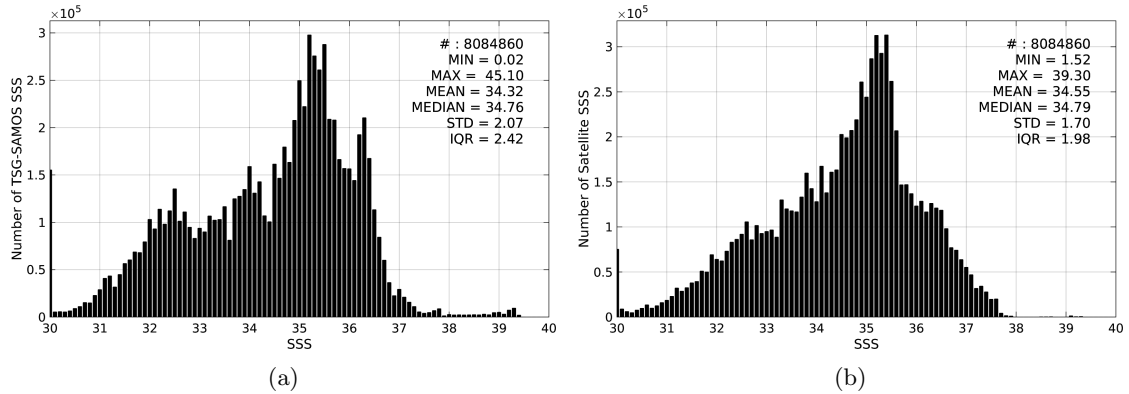
Figure 2: Histograms of SSS from TSG-SAMOS (a) and SMOS-L4-CATDS-CECOS-IFREMER-V2-WEEKLY-0.5DEG (b) considering all match-up pairs per bins of 0.1 over the Global Ocean Pi-MEP region and for the full satellite product period.
