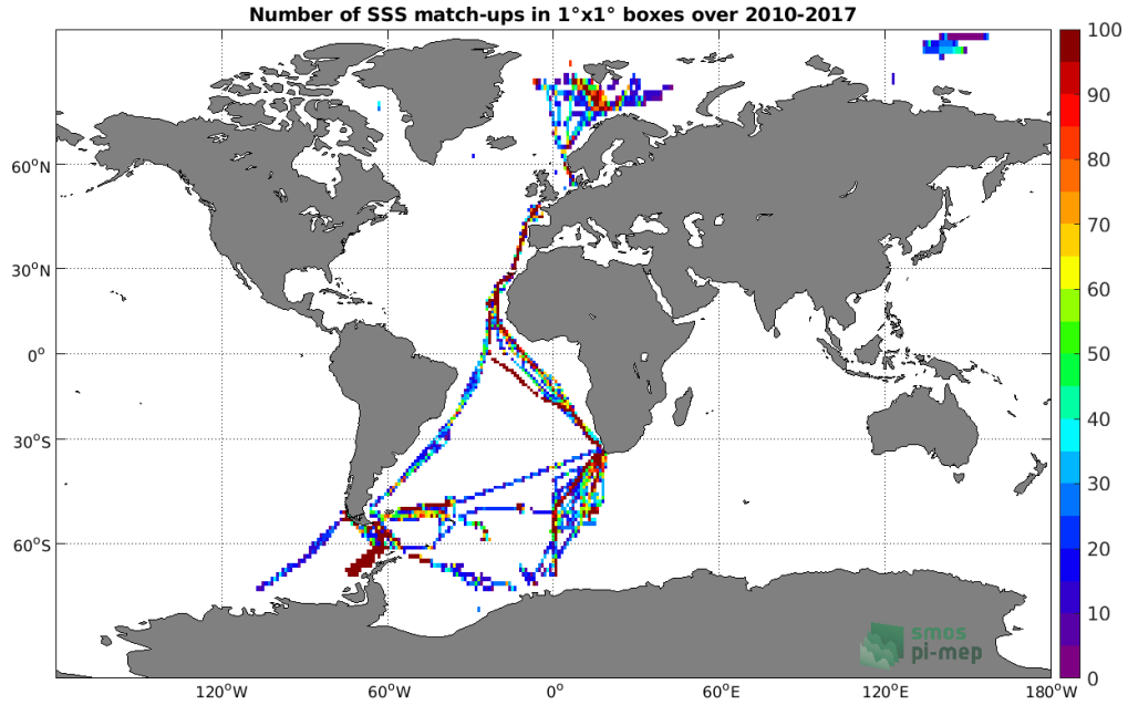
Figure 4: Number of SSS match-ups between TSG (Polarstern) SSS and the SMOS L4 v2 Weekly (CATDS-CECOS-IFREMER) SSS product for the Global Ocean Pi-MEP region over 1^\circ \times 1^\circ boxes and for the full satellite product period.
