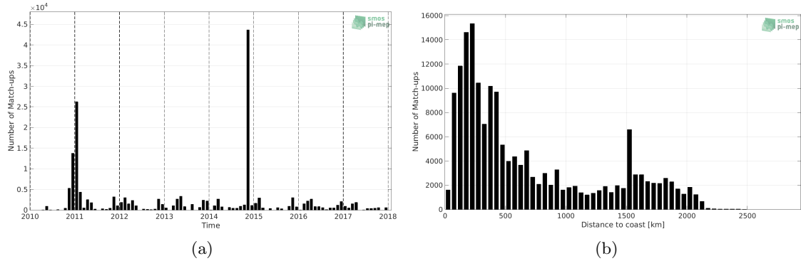
Figure 1: Number of match-ups between TSG (Polarstern) and SMOS L4 v2 Weekly (CATDS-CECOS-IFREMER) SSS as a function of time (a) and as function of the distance to coast (b) over the Global Ocean Pi-MEP region and for the full satellite product period.
