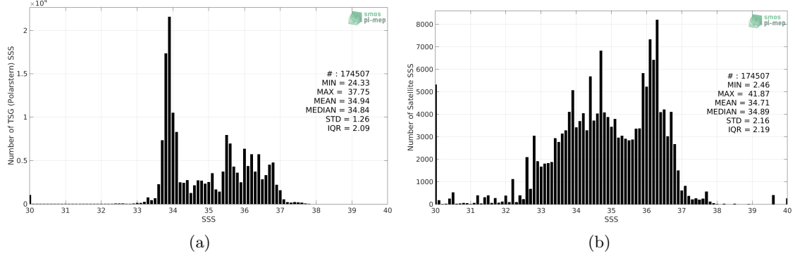
Figure 2: Histograms of SSS from TSG (Polarstern) (a) and SMOS L4 v2 Weekly (CATDS-CECOS-IFREMER) (b) considering all match-up pairs per bins of 0.1 over the Global Ocean Pi-MEP region and for the full satellite product period.
