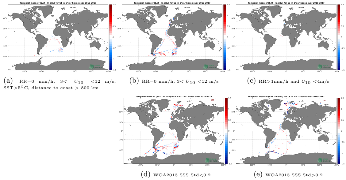
Figure 12: Temporal mean gridded over spatial boxes of size 1^\circ \times 1^\circ of \Delta SSS (SMOS L4 v2 Weekly (CATDS-CECOS-IFREMER) - TSG (Polarstern)) for 5 different subdatasets corresponding to:RR=0 mm/h, 3 < U_{10} < 12 m/s, SST>5°C, distance to coast > 800 km (a), RR=0 mm/h, 3 < U_{10} < 12 m/s (b), RR>1mm/h and U_{10} < 4 m/s (c), WOA2013 SSS Std<0.2 (d), WOA2013 SSS Std>0.2 (e).
