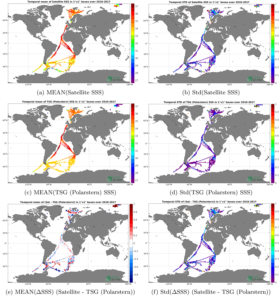
Figure 6: Temporal mean (left) and Std (right) of SSS from SMOS L4 v2 Weekly (CATDS-CECOS-IFREMER) (top), TSG (Polarstern) (middle), and of \Delta SSS (Satellite - TSG (Polarstern)). Only match-up pairs are used to generate these maps.
