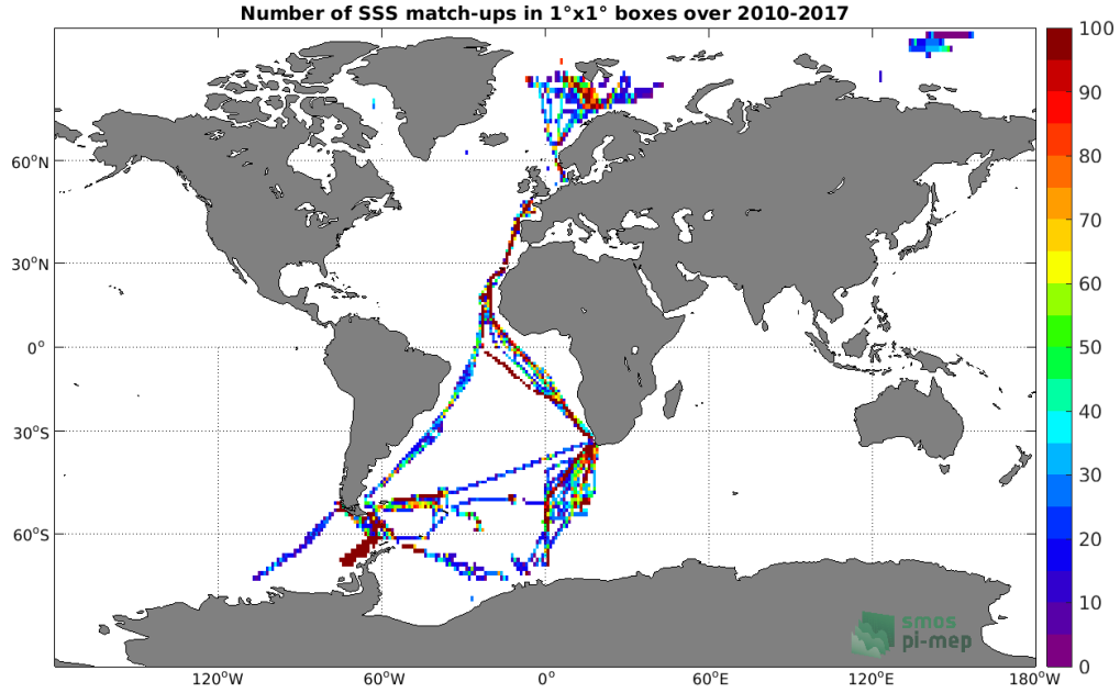
Figure 4: Number of SSS match-ups between TSG (Polarstern) SSS and the SMOS L4 v2 Weekly (CATDS-CECOS-IFREMER) SSS product for the Global Ocean Pi-MEP region over 1^\circ \times 1^\circ boxes and for the full satellite product period.
