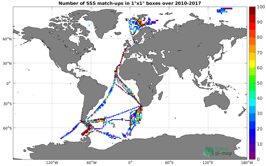
Figure 4: Number of SSS match-ups between TSG-POLARSTERN SSS and the SMOS-L4-CATDS-CECOS-IFREMER-V2-WEEKLY-0.5DEG SSS product for the Global Ocean Pi-MEP region over 1^\circ \times 1^\circ boxes and for the full satellite product period.
