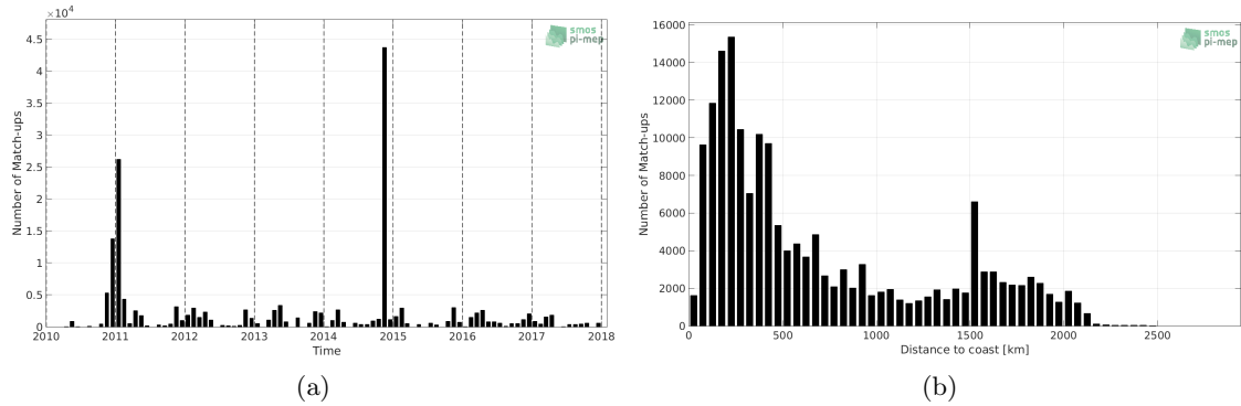
Figure 1: Number of match-ups between TSG-POLARSTERN and SMOS-L4-CATDS-CECOS-IFREMER-V2-WEEKLY-0.5DEG SSS as a function of time (a) and as function of the distance to coast (b) over the Global Ocean Pi-MEP region and for the full satellite product period.
