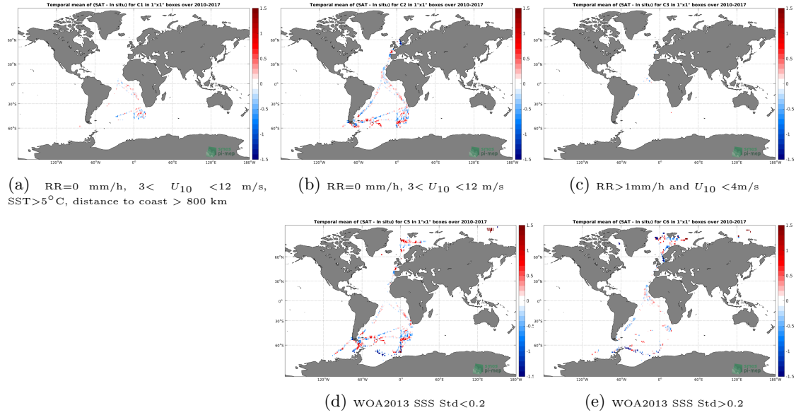
Figure 12: Temporal mean gridded over spatial boxes of size 1^\circ \times 1^\circ of \Delta SSS (SMOS-L4-CATDS-CECOS-IFREMER-V2-WEEKLY-0.5DEG - TSG-POLARSTERN) for 5 different subdatasets corresponding to: RR=0 mm/h, 3 < U_{10} < 12 m/s, SST > 5^\circ C , distance to coast > 800 km (a), RR=0 mm/h, 3 < U_{10} < 12 m/s (b), RR > 1 mm/h and U_{10} < 4 m/s (c), WOA2013 SSS Std < 0.2 (d), WOA2013 SSS Std > 0.2 (e).
