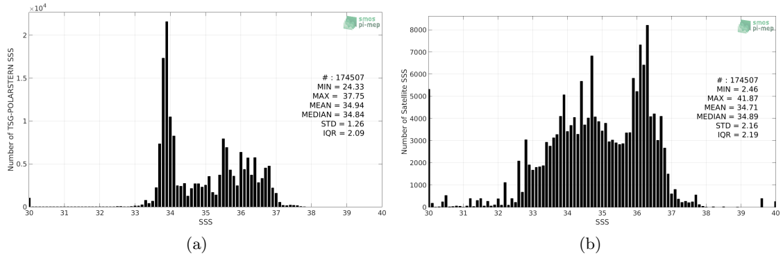
Figure 2: Histograms of SSS from TSG-POLARSTERN (a) and SMOS-L4-CATDS-CECOS-IFREMER-V2-WEEKLY-0.5DEG (b) considering all match-up pairs per bins of 0.1 over the Global Ocean Pi-MEP region and for the full satellite product period.
