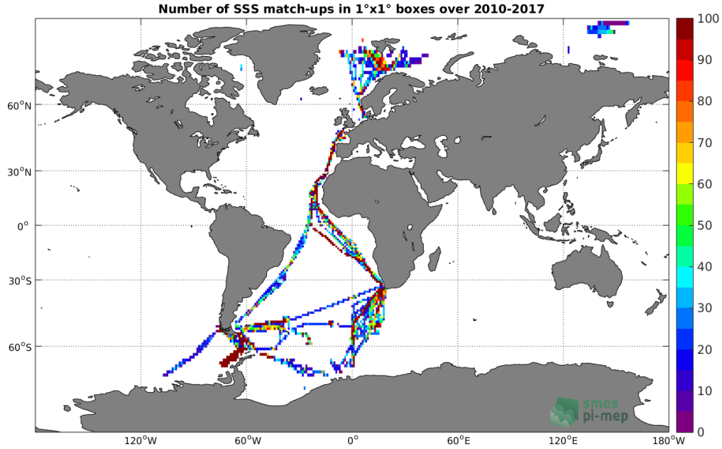
Figure 4: Number of SSS match-ups between TSG-POLARSTERN SSS and the SMOS-L4-CATDS-CECOS-IFREMER-V2-WEEKLY-0.5DEG SSS product for the Global Ocean Pi-MEP region over 1°x1° boxes and for the full satellite product period.
