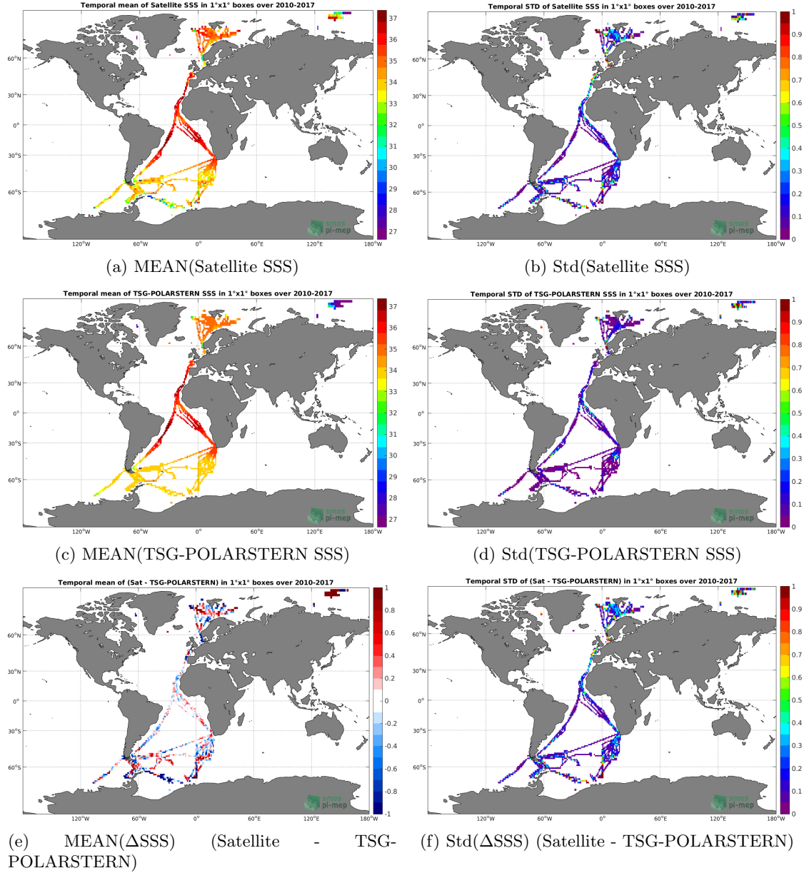
Figure 6: Temporal mean (left) and Std (right) of SSS from SMOS-L4-CATDS-CECOS-IFREMER-V2-WEEKLY-0.5DEG (top), TSG-POLARSTERN (middle), and of \Delta SSS (Satellite - TSG-POLARSTERN). Only match-up pairs are used to generate these maps.
