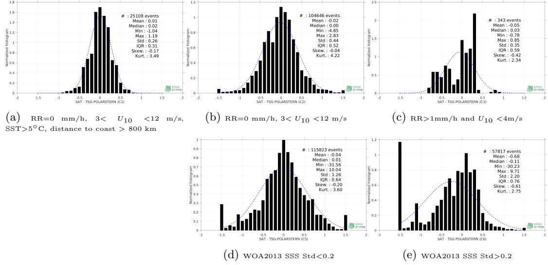
Figure 13: Normalized histogram of \Delta SSS (SMOS-L4-CATDS-CECOS-IFREMER-V2-WEEKLY-0.5DEG - TSG-POLARSTERN) for 5 different subdatasets corresponding to: RR=0 mm/h, 3 < U_{10} < 12 m/s, SST>5°C, distance to coast > 800 km (a), RR=0 mm/h, 3 < U_{10} < 12 m/s (b), RR>1mm/h and U_{10} < 4 m/s (c), WOA2013 SSS Std<0.2 (d), WOA2013 SSS Std>0.2 (e).
