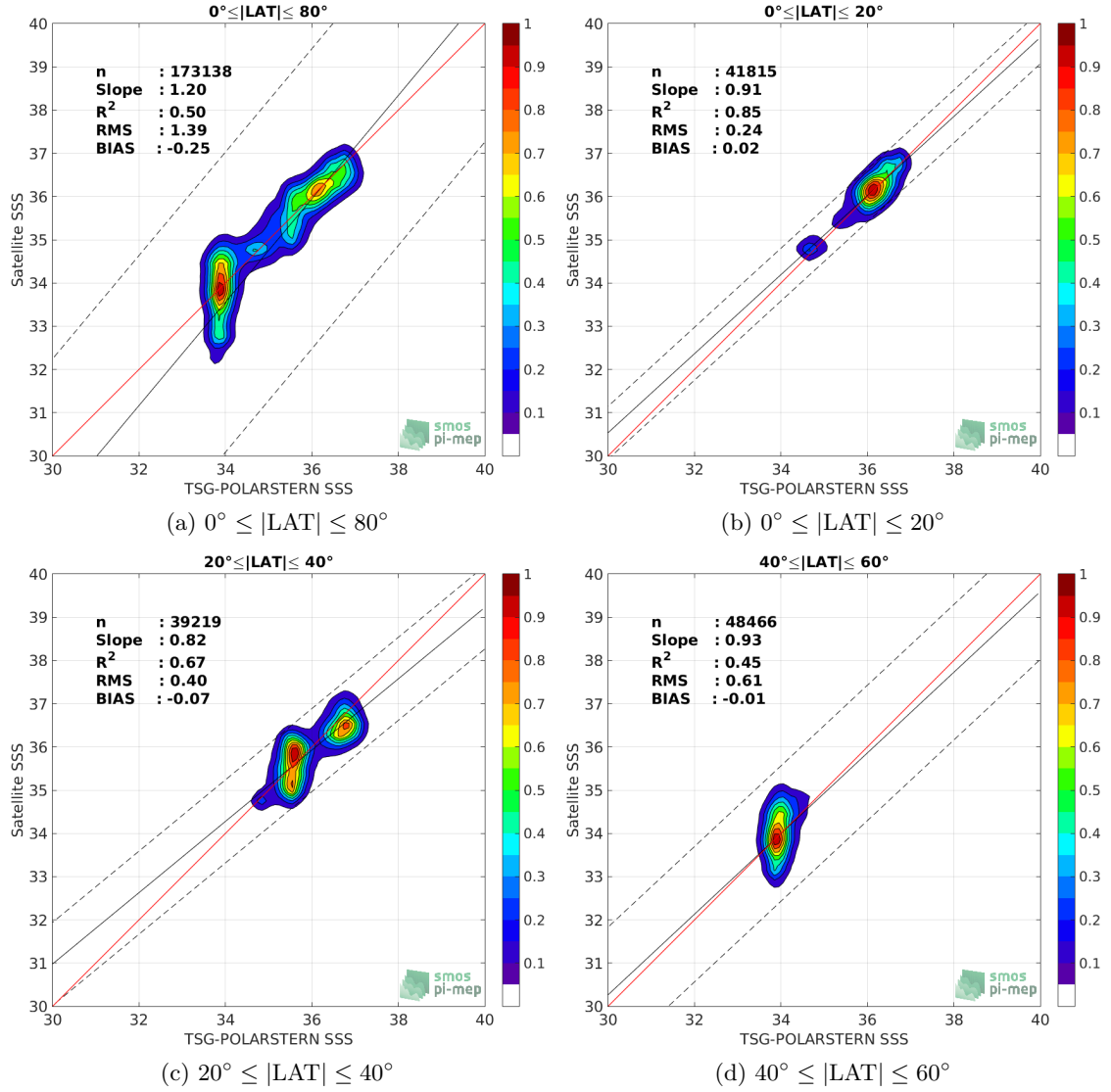
Figure 9: Contour maps of the concentration of SMOS-L4-CATDS-CECOS-IFREMER-V2-WEEKLY-0.5DEG SSS (y-axis) versus TSG-POLARSTERN SSS (x-axis) at match-up pairs for different latitude bands. For each plot, the red line shows x=y . The black thin and dashed lines indicate a linear fit through the data cloud and the \pm 95\% confidence levels, respectively. The number match-up pairs n , the slope and R^2 coefficient of the linear fit, the root mean square (RMS) and the mean bias between satellite and in situ data are indicated for each latitude band in each plots.
