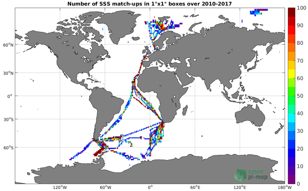
Figure 4: Number of SSS match-ups between TSG-POLARSTERN SSS and the SMOS-L4-CATDS-CECOS-IFREMER-V2-WEEKLY-0.5DEG SSS product for the Global Ocean Pi-MEP region over 1^\circ \times 1^\circ boxes and for the full satellite product period.
