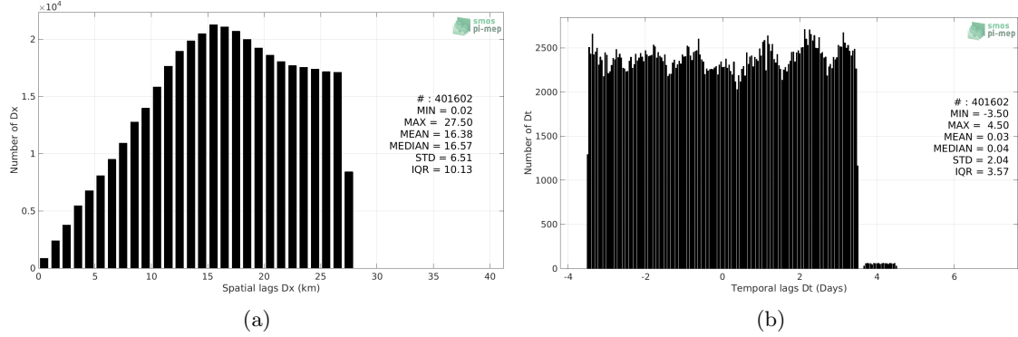
Figure 5: Histograms of the spatial (a) and temporal (b) lags between the time of the TSG (LEGOS-Survostral) measurements and the date of the corresponding SMOS L4 v2 Weekly (CATDS-CECOS-IFREMER) SSS product.
