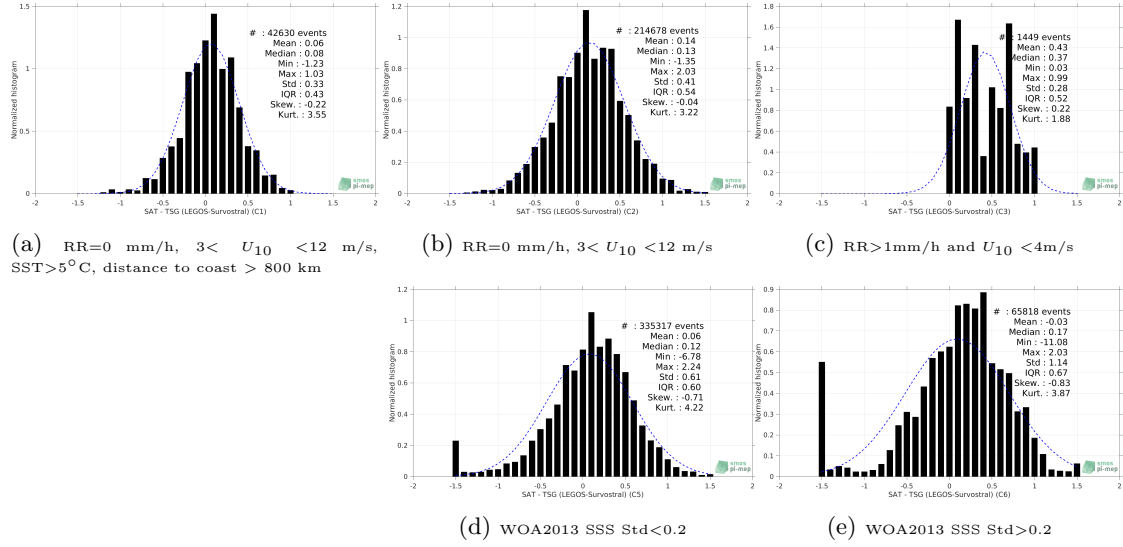
Figure 13: Normalized histogram of \Delta SSS (SMOS L4 v2 Weekly (CATDS-CECOS-IFREMER) - TSG (LEGOS-Survostral)) for 5 different subdatasets corresponding to: RR=0 mm/h, 3 < U_{10} < 12 m/s, SST > 5°C, distance to coast > 800 km (a), RR=0 mm/h, 3 < U_{10} < 12 m/s (b), RR > 1mm/h and U_{10} < 4 m/s (c), WOA2013 SSS Std < 0.2 (d), WOA2013 SSS Std > 0.2 (e).
