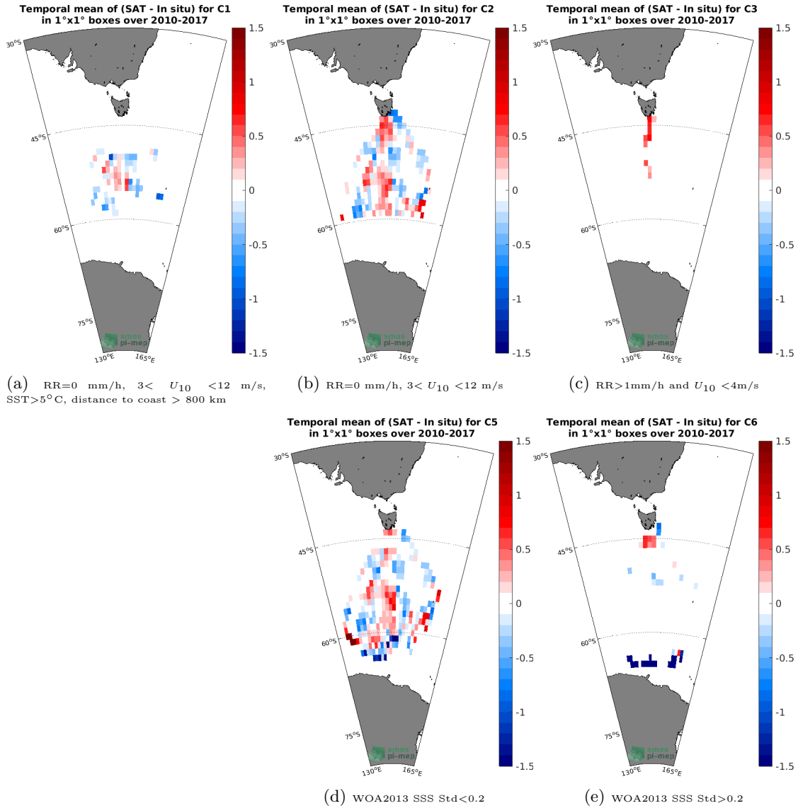
Figure 12: Temporal mean gridded over spatial boxes of size 1°x1° of \Delta SSS (SMOS L4 v2 Weekly (CATDS-CECOS-IFREMER) - TSG (LEGOS-Survostral)) for 5 different subdatasets corresponding to:RR=0 mm/h, 3 < U_{10} < 12 m/s, SST>5°C, distance to coast > 800 km (a), RR=0 mm/h, 3 < U_{10} < 12 m/s (b), RR>1mm/h and U_{10} < 4 m/s (c), WOA2013 SSS Std<0.2 (d), WOA2013 SSS Std>0.2 (e).
