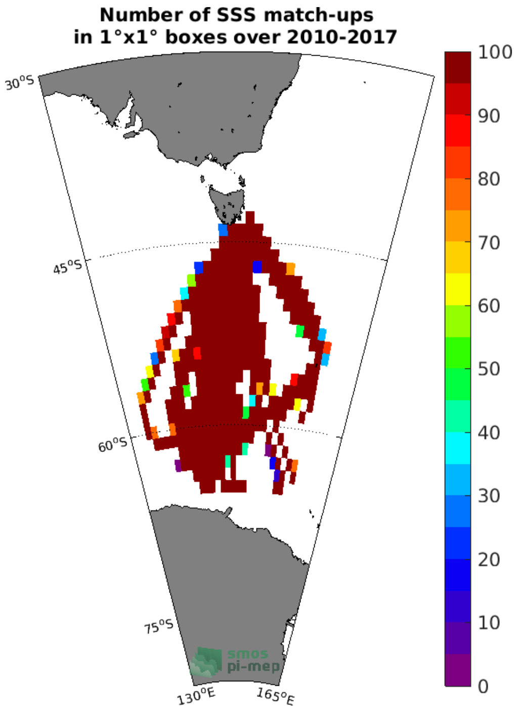
Figure 4: Number of SSS match-ups between TSG (LEGOS-Survostral) SSS and the SMOS L4 v2 Weekly (CATDS-CECOS-IFREMER) SSS product for the Global Ocean Pi-MEP region over 1°x1° boxes and for the full satellite product period.
