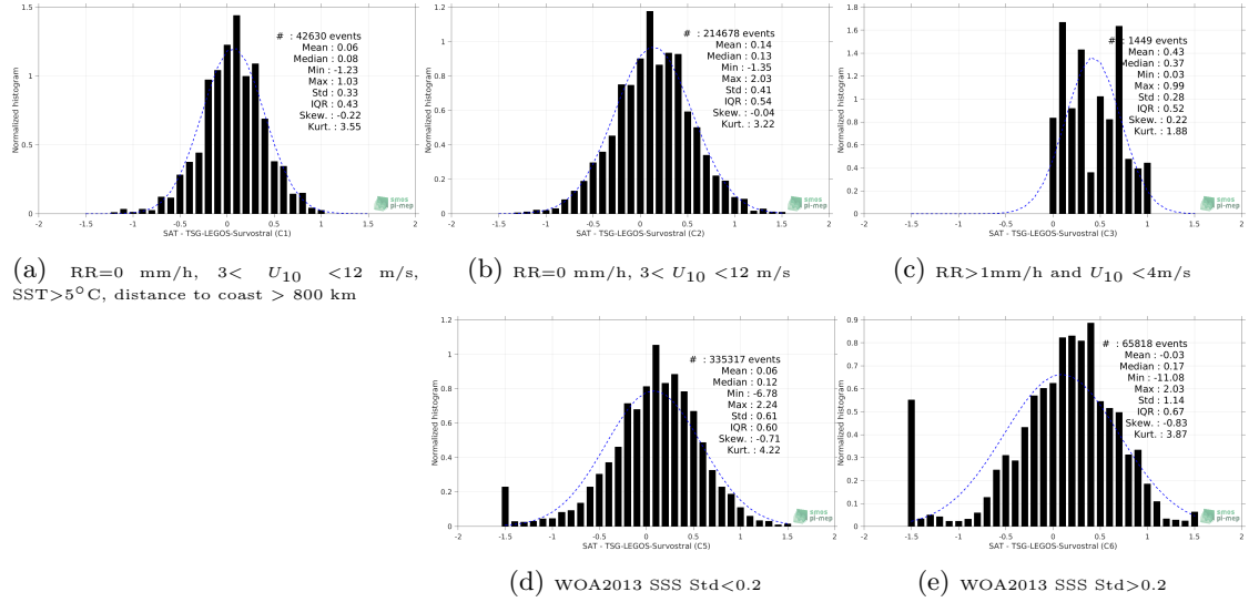
Figure 13: Normalized histogram of \Delta SSS (SMOS-L4-CATDS-CECOS-IFREMER-V2-WEEKLY-0.5DEG - TSG-LEGOS-Survostral) for 5 different subdatasets corresponding to: RR=0 mm/h, 3 < U_{10} < 12 m/s, SST>5°C, distance to coast > 800 km (a), RR=0 mm/h, 3 < U_{10} < 12 m/s (b), RR>1mm/h and U_{10} < 4 m/s (c), WOA2013 SSS Std<0.2 (d), WOA2013 SSS Std>0.2 (e).
