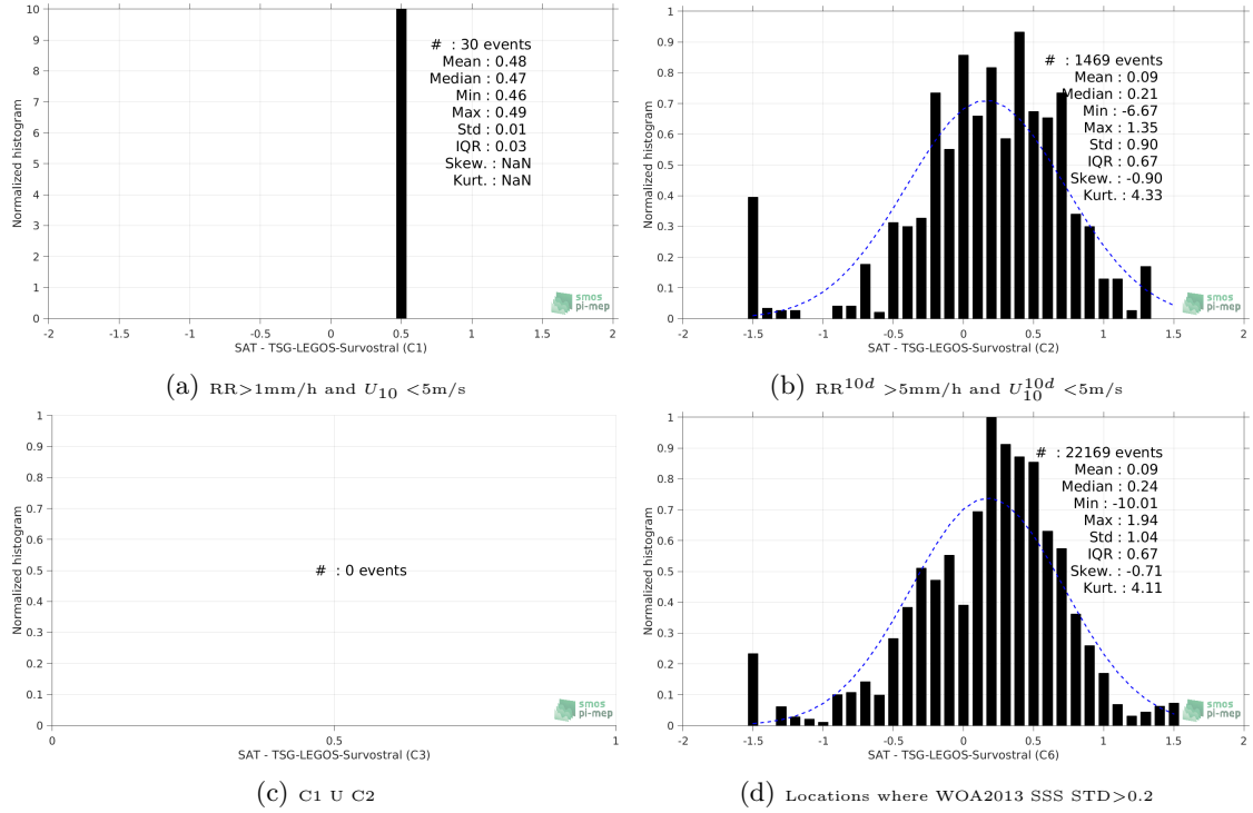
Figure 13: Normalized histogram of \Delta\text{SSS} (SMOS-L4-CATDS-CECOS-IFREMER-V2-WEEKLY-0.5DEG - TSG-LEGOS-Survostral) for 6 different subdatasets corresponding to: RR > 1\text{mm/h} and U_{10} < 5\text{m/s} (a), RR^{10d} > 5\text{mm/h} and U_{10}^{10d} < 5\text{m/s} (b), C1 U C2 (c), Locations where WOA2013 SSS STD > 0.2 (d).
