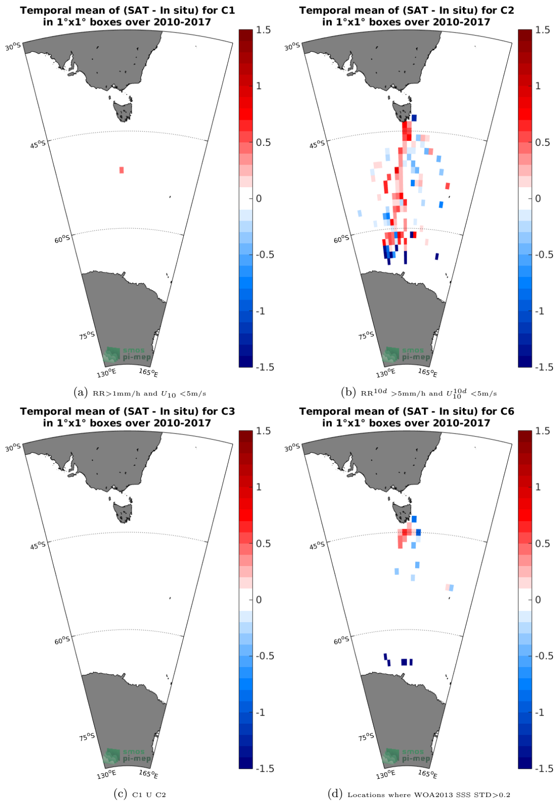
Figure 12: Temporal mean gridded over spatial boxes of size 1°x1° of \Delta SSS (SMOS-L4-CATDS-CECOS-IFREMER-V2-WEEKLY-0.5DEG - TSG-LEGOS-Survostral) for 4 different subdatasets corresponding to: RR > 1\text{mm/h} and U_{10} < 5\text{m/s} (a), RR^{10d} > 5\text{mm/h} and U_{10}^{10d} < 5\text{m/s} (b), C1 U C2 (c), Locations where WOA2013 SSS STD > 0.2 (d).
