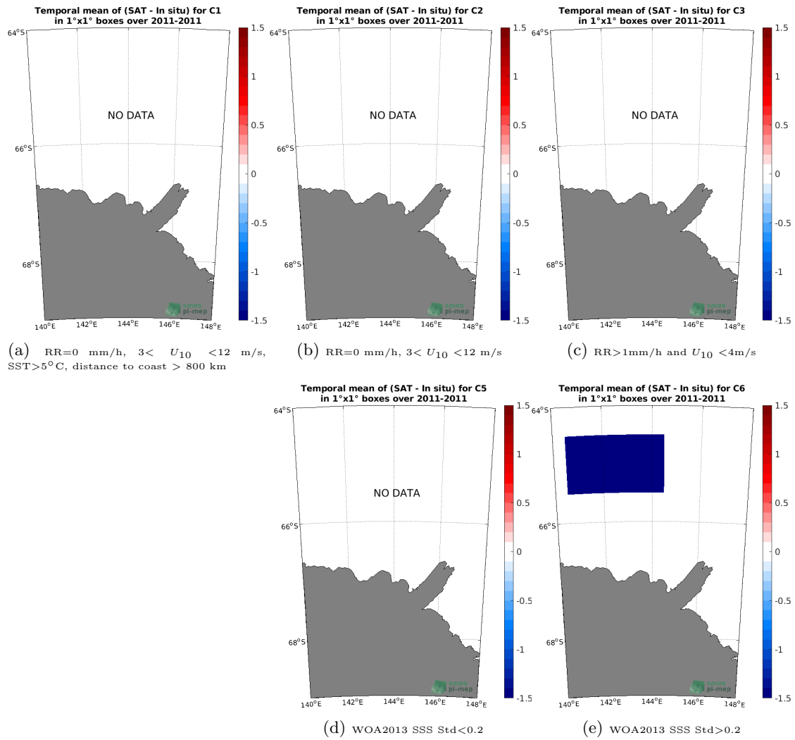
Figure 12: Temporal mean gridded over spatial boxes of size 1°x1° of \Delta SSS (SMOS L4 v2 Weekly (CATDS-CECOS-IFREMER) - TSG (LEGOS-Surv-Adel)) for 5 different subdatasets corresponding to:RR=0 mm/h, 3 < U_{10} < 12 m/s, SST>5°C, distance to coast > 800 km (a), RR=0 mm/h, 3 < U_{10} < 12 m/s (b), RR>1mm/h and U_{10} < 4 m/s (c), WOA2013 SSS Std<0.2 (d), WOA2013 SSS Std>0.2 (e).
