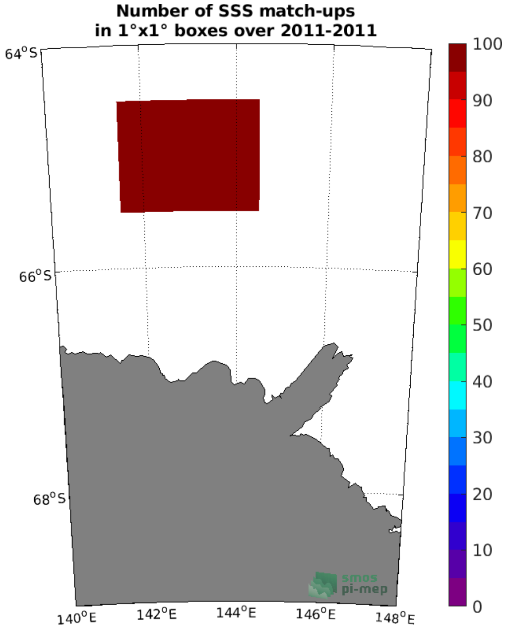
Figure 4: Number of SSS match-ups between TSG (LEGOS-Surv-Adel) SSS and the SMOS L4 v2 Weekly (CATDS-CECOS-IFREMER) SSS product for the Global Ocean Pi-MEP region over 1^\circ \times 1^\circ boxes and for the full satellite product period.
