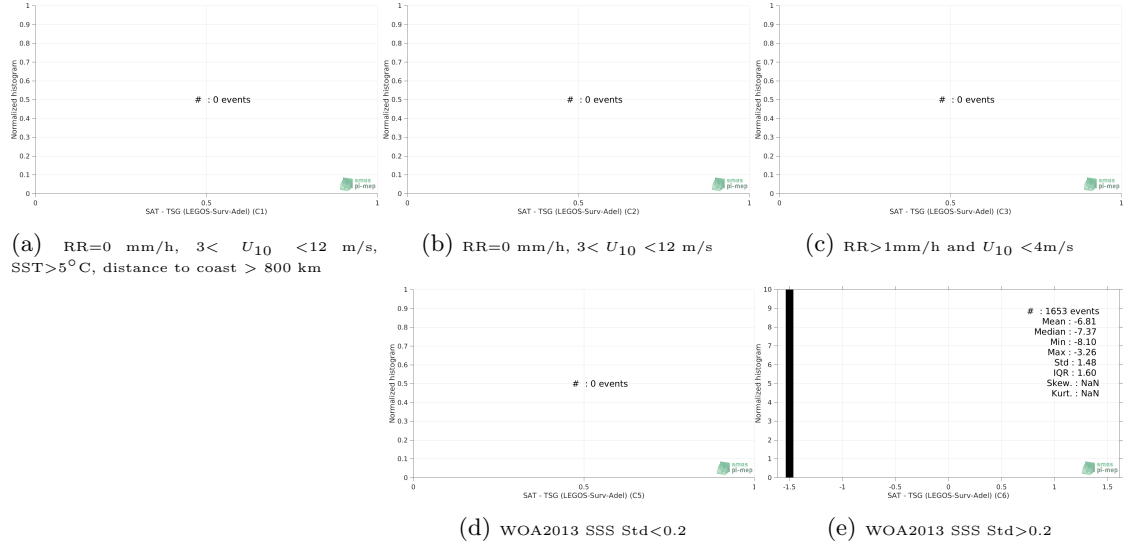
Figure 13: Normalized histogram of \Delta\text{SSS} (SMOS L4 v2 Weekly (CATDS-CECOS-IFREMER) - TSG (LEGOS-Surv-Adel)) for 5 different subdatasets corresponding to: RR=0 mm/h, 3 < U_{10} < 12 m/s, SST > 5^\circ\text{C} , distance to coast > 800 km (a), RR=0 mm/h, 3 < U_{10} < 12 m/s (b), RR > 1\text{mm/h} and U_{10} < 4\text{m/s} (c), WOA2013 SSS Std < 0.2 (d), WOA2013 SSS Std > 0.2 (e).
