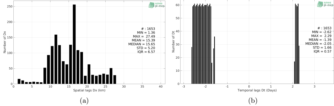
Figure 5: Histograms of the spatial (a) and temporal (b) lags between the location/time of the TSG (LEGOS-Surv-Adel) measurement and the date of the corresponding SMOS L4 v2 Weekly (CATDS-CECOS-IFREMER) SSS pixel.
