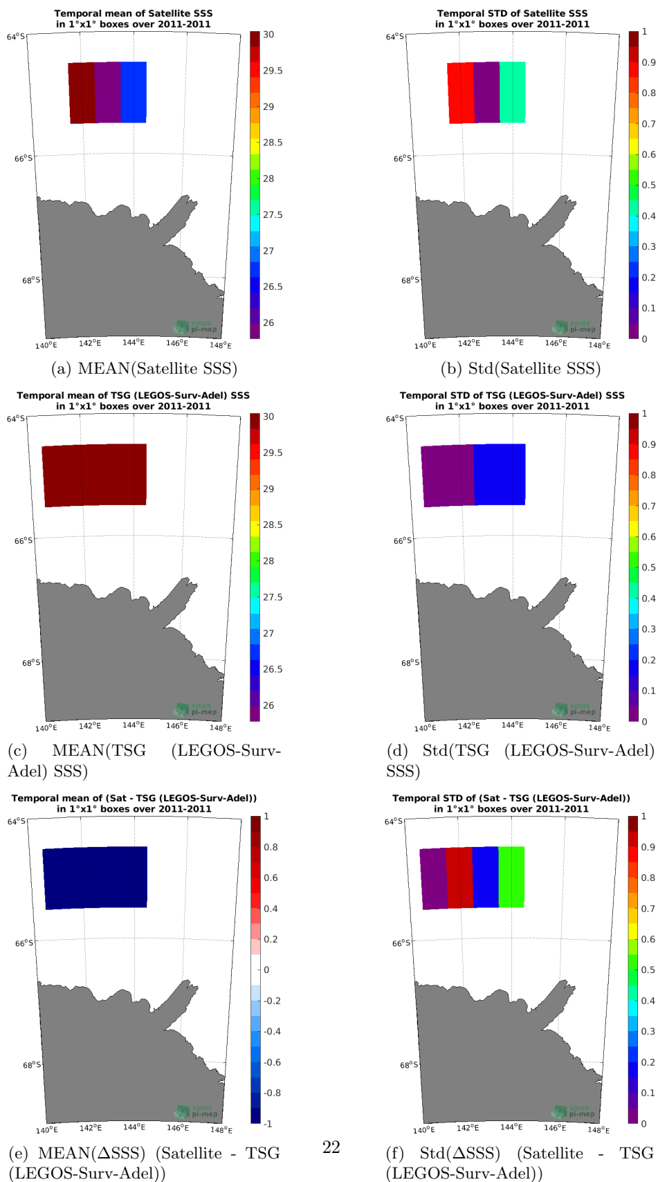
Figure 6: Temporal mean (left) and Std (right) of SSS from SMOS L4 v2 Weekly (CATDS-CECOS-IFREMER) (top), TSG (LEGOS-Surv-Adel) (middle), and of \Delta SSS (Satellite - TSG (LEGOS-Surv-Adel)). Only match-up pairs are used to generate these maps.
