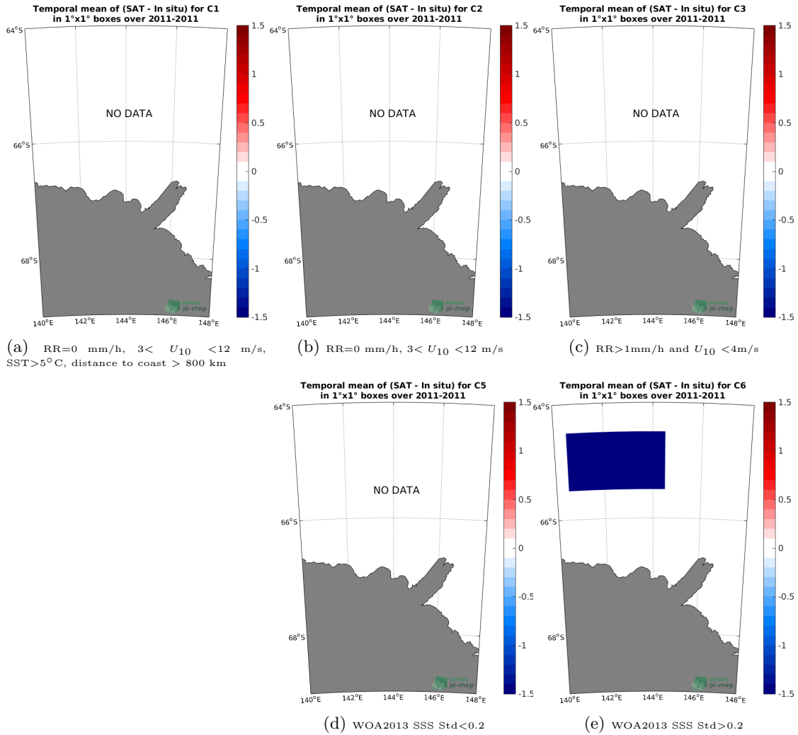
Figure 12: Temporal mean gridded over spatial boxes of size 1°x1° of \Delta SSS (SMOS-L4-CATDS-CECOS-IFREMER-V2-WEEKLY-0.5DEG - TSG-LEGOS-Surv-Adel) for 5 different subdatasets corresponding to:RR=0 mm/h, 3 < U_{10} < 12 m/s, SST>5°C, distance to coast > 800 km (a), RR=0 mm/h, 3 < U_{10} < 12 m/s (b), RR>1mm/h and U_{10} < 4 m/s (c), WOA2013 SSS Std<0.2 (d), WOA2013 SSS Std>0.2 (e).
