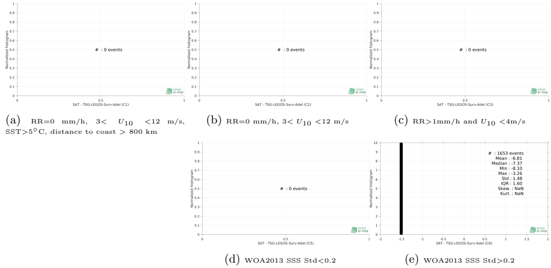
Figure 13: Normalized histogram of \Delta SSS (SMOS-L4-CATDS-CECOS-IFREMER-V2-WEEKLY-0.5DEG - TSG-LEGOS-Surv-Adel) for 5 different subdatasets corresponding to: RR=0 mm/h, 3 < U_{10} < 12 m/s, SST>5°C, distance to coast > 800 km (a), RR=0 mm/h, 3 < U_{10} < 12 m/s (b), RR>1mm/h and U_{10} < 4 m/s (c), WOA2013 SSS Std<0.2 (d), WOA2013 SSS Std>0.2 (e).
