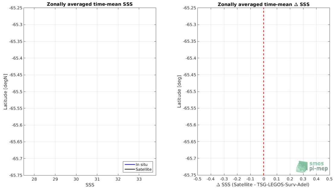
Figure 8: Left panel: Zonal mean SSS from SMOS-L4-CATDS-CECOS-IFREMER-V2-WEEKLY-0.5DEG satellite product (black) and from TSG-LEGOS-Surv-Adel (blue). Right panel: Zonal mean of \Delta SSS (Satellite - TSG-LEGOS-Surv-Adel) for all the collected Pi-MEP match-up pairs estimated over the full satellite product period.
