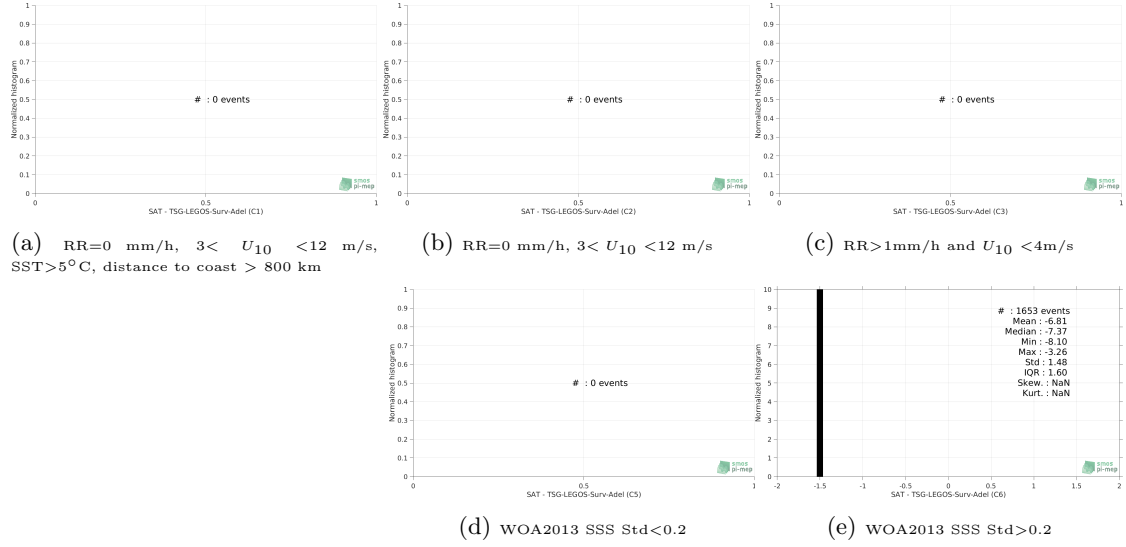
Figure 13: Normalized histogram of \Delta\text{SSS} (SMOS-L4-CATDS-CECOS-IFREMER-V2-WEEKLY-0.5DEG - TSG-LEGOS-Surv-Adel) for 5 different subdatasets corresponding to: RR=0 mm/h, 3 < U_{10} < 12 m/s, SST > 5^\circ\text{C} , distance to coast > 800 km (a), RR=0 mm/h, 3 < U_{10} < 12 m/s (b), RR > 1\text{mm/h} and U_{10} < 4\text{m/s} (c), WOA2013 SSS Std < 0.2 (d), WOA2013 SSS Std > 0.2 (e).
