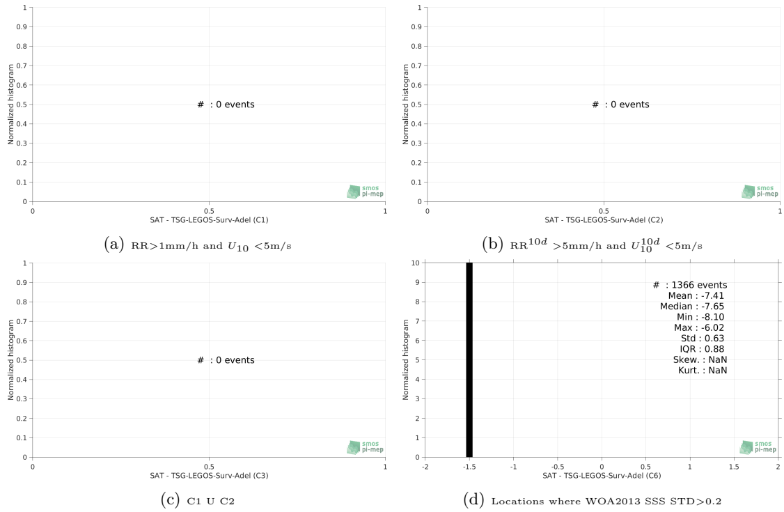
Figure 13: Normalized histogram of \Delta\text{SSS} (SMOS-L4-CATDS-CECOS-IFREMER-V2-WEEKLY-0.5DEG - TSG-LEGOS-Surv-Adel) for 6 different subdatasets corresponding to: RR > 1\text{mm/h} and U_{10} < 5\text{m/s} (a), RR^{10d} > 5\text{mm/h} and U_{10}^{10d} < 5\text{m/s} (b), C1 U C2 (c), Locations where WOA2013 SSS STD > 0.2 (d).
