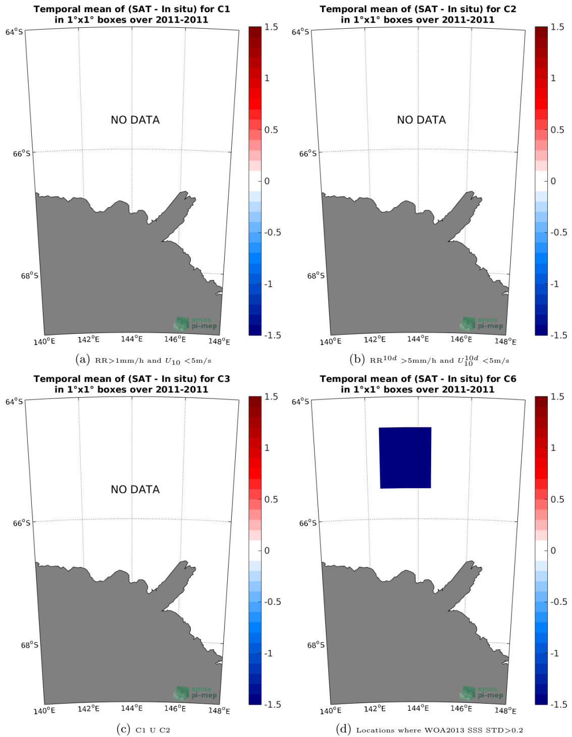
Figure 12: Temporal mean gridded over spatial boxes of size 1^\circ \times 1^\circ of \Delta\text{SSS} (SMOS-L4-CATDS-CECOS-IFREMER-V2-WEEKLY-0.5DEG - TSG-LEGOS-Surv-Adel) for 4 different subdatasets corresponding to: RR > 1\text{mm/h} and U_{10} < 5\text{m/s} (a), RR^{10d} > 5\text{mm/h} and U_{10}^{10d} < 5\text{m/s} (b), C1 U C2 (c), Locations where WOA2013 SSS STD > 0.2 (d).
