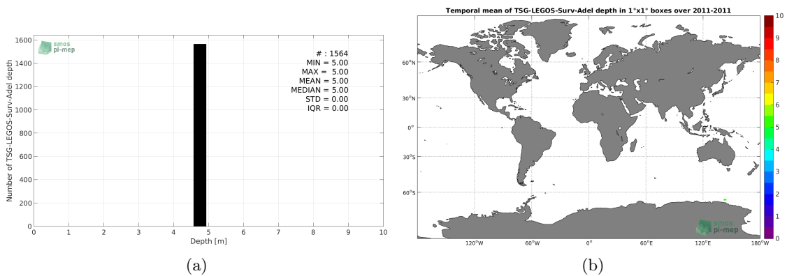
Figure 3: Histograms of the depth of the upper level SSS measurements from TSG-LEGOS-Surv-Adel in the Match-up DataBase for the Global Ocean Pi-MEP region (a) and temporal mean spatial distribution of pressure of the in situ SSS data over 1^\circ \times 1^\circ boxes and for the full satellite product period (b).
