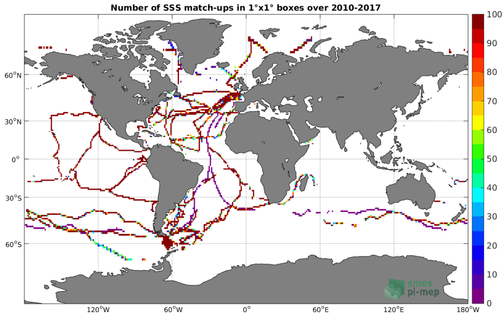
Figure 4: Number of SSS match-ups between TSG-GOSUD-Sailing-ship SSS and the SMOS-L4-CATDS-CECOS-IFREMER-V2-WEEKLY-0.5DEG SSS product for the Global Ocean Pi-MEP region over 1^\circ \times 1^\circ boxes and for the full satellite product period.
