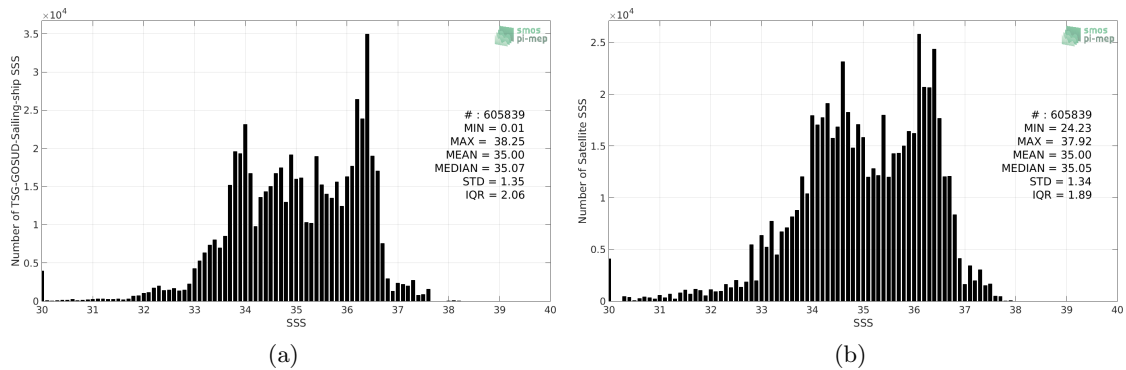
Figure 2: Histograms of SSS from TSG-GOSUD-Sailing-ship (a) and SMOS-L4-CATDS-CECOS-IFREMER-V2-WEEKLY-0.5DEG (b) considering all match-up pairs per bins of 0.1 over the Global Ocean Pi-MEP region and for the full satellite product period.
