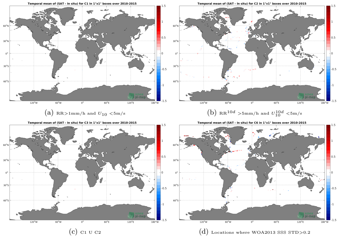
Figure 12: Temporal mean gridded over spatial boxes of size 1^\circ \times 1^\circ of \Delta SSS (SMOS-L4-CATDS-CECOS-IFREMER-V2-WEEKLY-0.5DEG - TSG-GOSUD-Sailing-ship) for 4 different subdatasets corresponding to: RR > 1\text{mm/h} and U_{10} < 5\text{m/s} (a), RR^{10d} > 5\text{mm/h} and U_{10}^{10d} < 5\text{m/s} (b), C1 U C2 (c), Locations where WOA2013 SSS STD > 0.2 (d).
