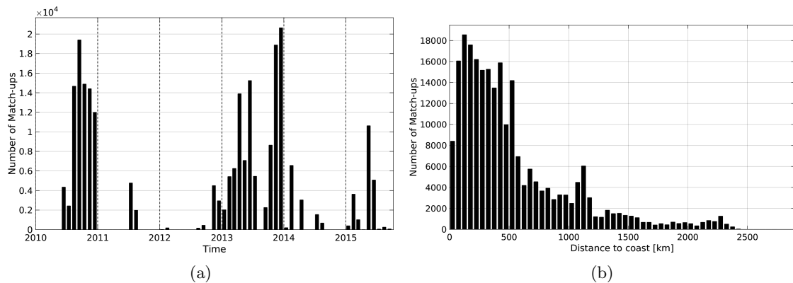
Figure 1: Number of match-ups between TSG-GOSUD-Sailing-ship and SMOS-L4-CATDS-CECOS-IFREMER-V2-WEEKLY-0.5DEG SSS as a function of time (a) and as function of the distance to coast (b) over the Global Ocean Pi-MEP region and for the full satellite product period.
