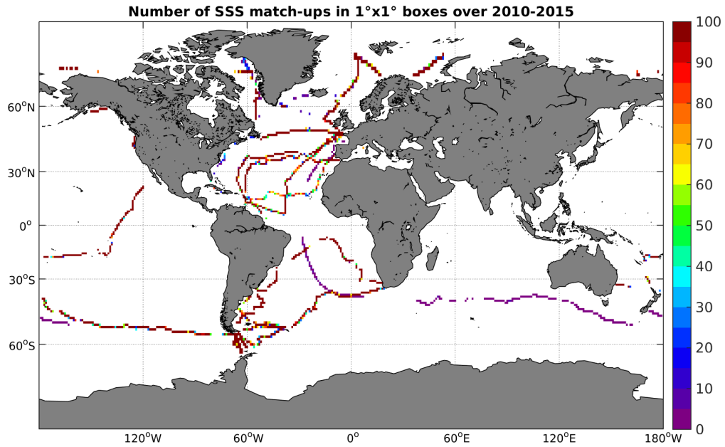
Figure 4: Number of SSS match-ups between TSG-GOSUD-Sailing-ship SSS and the SMOS-L4-CATDS-CECOS-IFREMER-V2-WEEKLY-0.5DEG SSS product for the Global Ocean Pi-MEP region over 1°x1° boxes and for the full satellite product period.
