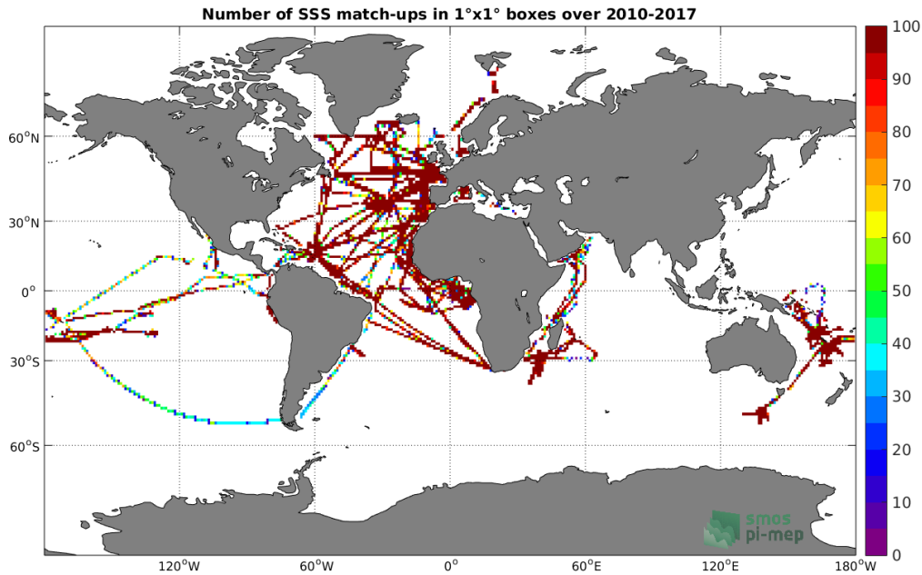
Figure 4: Number of SSS match-ups between TSG-GOSUD-Research-vessel SSS and the SMOS-L4-CATDS-CECOS-IFREMER-V2-WEEKLY-0.5DEG SSS product for the Global Ocean Pi-MEP region over 1°x1° boxes and for the full satellite product period.
