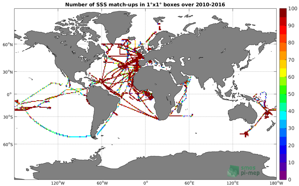
Figure 4: Number of SSS match-ups between TSG-GOSUD-Research-vessel SSS and the SMOS-L4-CATDS-CECOS-IFREMER-V2-WEEKLY-0.5DEG SSS product for the Global Ocean Pi-MEP region over 1^\circ \times 1^\circ boxes and for the full satellite product period.
