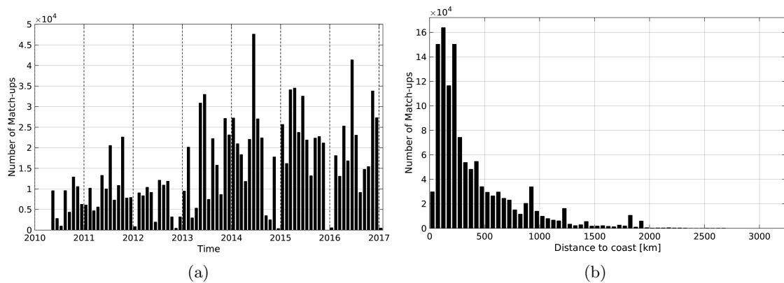
Figure 1: Number of match-ups between TSG-GOSUD-Research-vessel and SMOS-L4-CATDS-CECOS-IFREMER-V2-WEEKLY-0.5DEG SSS as a function of time (a) and as function of the distance to coast (b) over the Global Ocean Pi-MEP region and for the full satellite product period.
