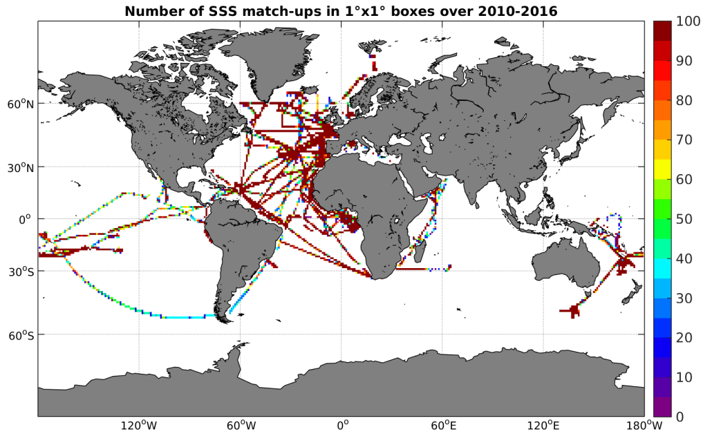
Figure 4: Number of SSS match-ups between TSG-GOSUD-Research-vessel SSS and the SMOS-L4-CATDS-CECOS-IFREMER-V2-WEEKLY-0.5DEG SSS product for the Global Ocean Pi-MEP region over 1°x1° boxes and for the full satellite product period.
