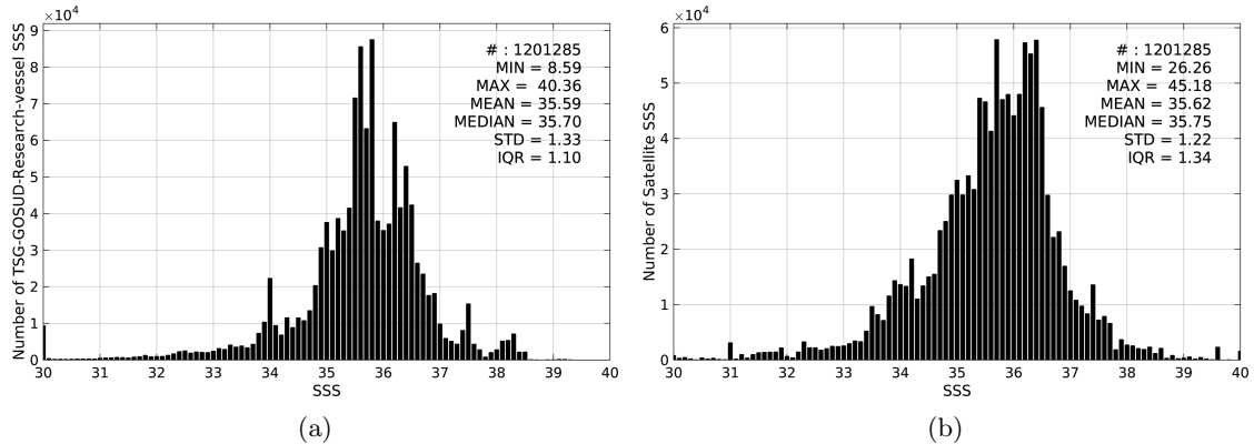
Figure 2: Histograms of SSS from TSG-GOSUD-Research-vessel (a) and SMOS-L4-CATDS-CECOS-IFREMER-V2-WEEKLY-0.5DEG (b) considering all match-up pairs per bins of 0.1 over the Global Ocean Pi-MEP region and for the full satellite product period.
