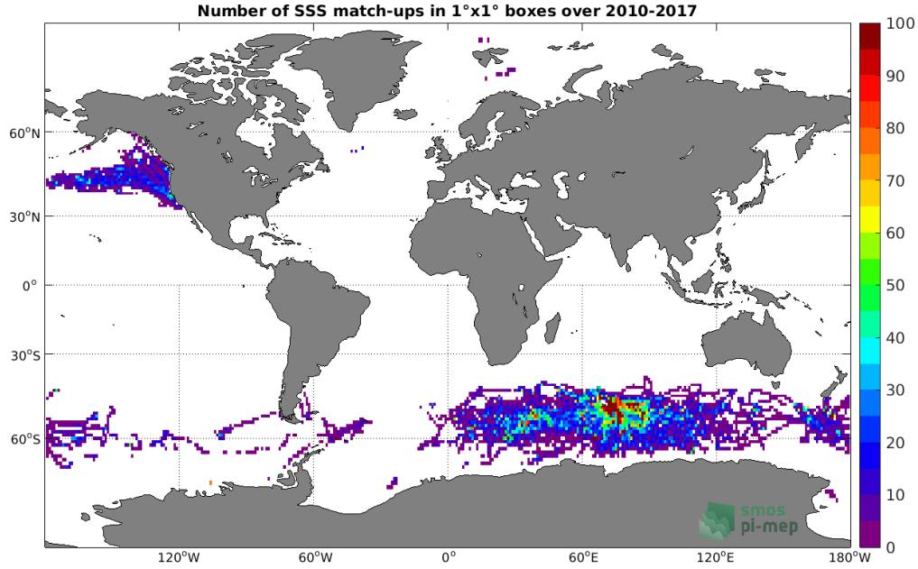
Figure 4: Number of SSS match-ups between Sea mammals SSS and the SMOS L4 v2 Weekly (CATDS-CECOS-IFREMER) SSS product for the Global Ocean Pi-MEP region over 1°x1° boxes and for the full satellite product period.
