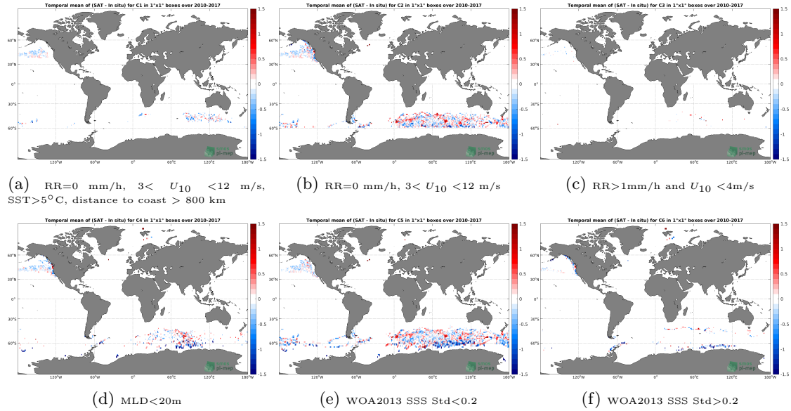
Figure 12: Temporal mean gridded over spatial boxes of size 1^\circ \times 1^\circ of \Delta SSS (SMOS L4 v2 Weekly (CATDS-CECOS-IFREMER) - Sea mammals) for 6 different subdatasets corresponding to: RR=0 mm/h, 3 < U_{10} < 12 m/s, SST > 5^\circ C , distance to coast > 800 km (a), RR=0 mm/h, 3 < U_{10} < 12 m/s (b), RR > 1 mm/h and U_{10} < 4 m/s (c), MLD < 20 m (d), WOA2013 SSS Std < 0.2 (e), WOA2013 SSS Std > 0.2 (f).
