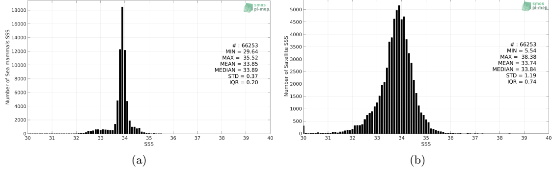
Figure 2: Histograms of SSS from Sea mammals (a) and SMOS L4 v2 Weekly (CATDS-CECOS-IFREMER) (b) considering all match-up pairs per bins of 0.1 over the Global Ocean Pi-MEP region and for the full satellite product period.
