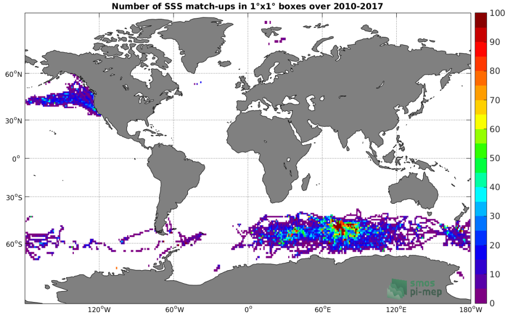
Figure 4: Number of SSS match-ups between Sea mammals SSS and the SMOS-L4-CATDS-CECOS-IFREMER-V2-WEEKLY-0.5DEG SSS product for the Global Ocean Pi-MEP region over 1°x1° boxes and for the full satellite product period.
