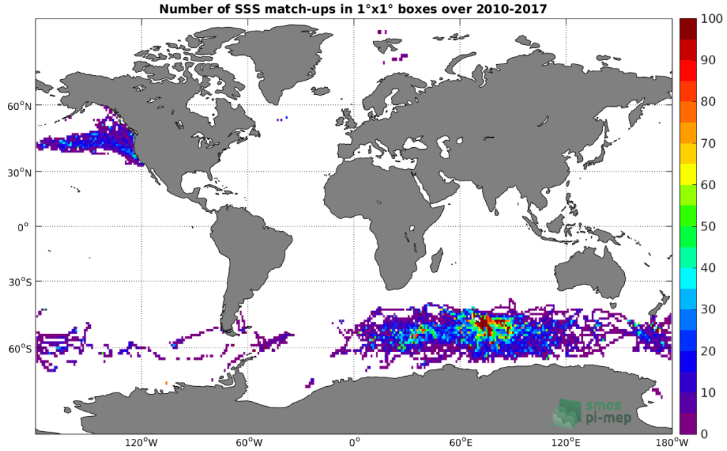
Figure 4: Number of SSS match-ups between Sea mammals SSS and the SMOS-L4-CATDS-CECOS-IFREMER-V2-WEEKLY-0.5DEG SSS product for the Global Ocean Pi-MEP region over 1°x1° boxes and for the full satellite product period.
