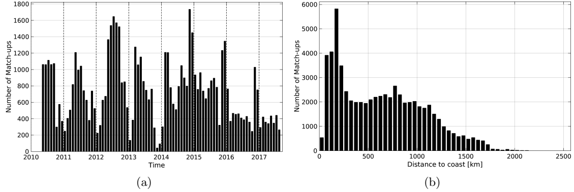
Figure 1: Number of match-ups between Sea mammals and SMOS-L4-CATDS-CECOS-IFREMER-V2-WEEKLY-0.5DEG SSS as a function of time (a) and as function of the distance to coast (b) over the Global Ocean Pi-MEP region and for the full satellite product period.
