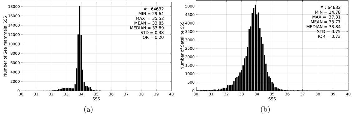
Figure 2: Histograms of SSS from Sea mammals (a) and SMOS-L4-CATDS-CECOS-IFREMER-V2-WEEKLY-0.5DEG (b) considering all match-up pairs per bins of 0.1 over the Global Ocean Pi-MEP region and for the full satellite product period.
