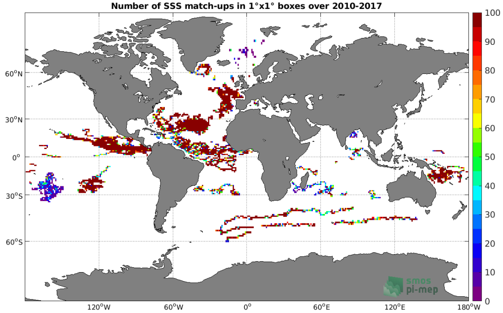
Figure 3: Number of SSS match-ups between Surface drifters SSS and the SMOS L4 v2 Weekly (CATDS-CECOS-IFREMER) SSS product for the Global Ocean Pi-MEP region over 1^\circ \times 1^\circ boxes and for the full satellite product period.
