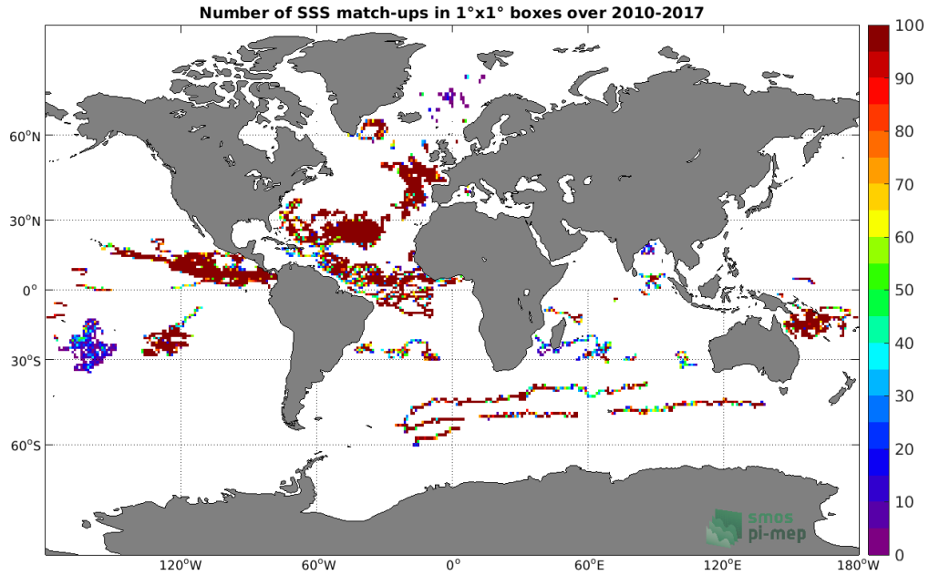
Figure 3: Number of SSS match-ups between Surface drifters SSS and the SMOS L4 v2 Weekly (CATDS-CECOS-IFREMER) SSS product for the Global Ocean Pi-MEP region over 1°x1° boxes and for the full satellite product period.
