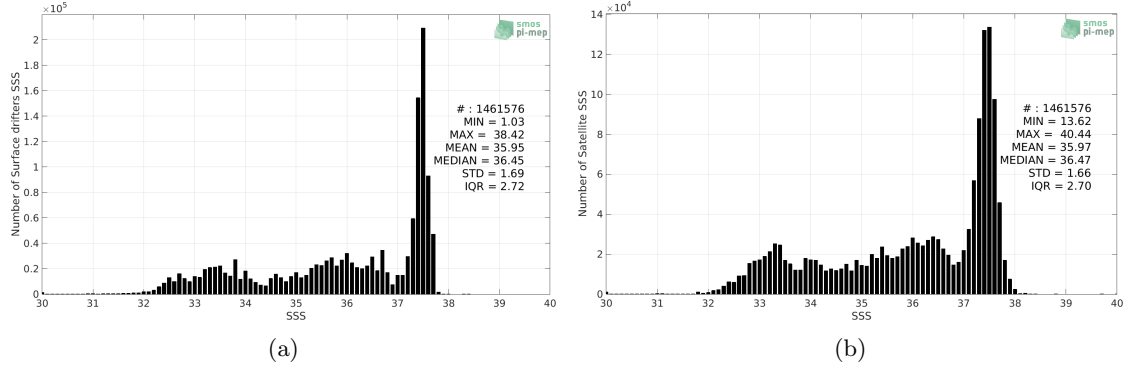
Figure 2: Histograms of SSS from Surface drifters (a) and SMOS L4 v2 Weekly (CATDS-CECOS-IFREMER) (b) considering all match-up pairs per bins of 0.1 over the Global Ocean Pi-MEP region and for the full satellite product period.
