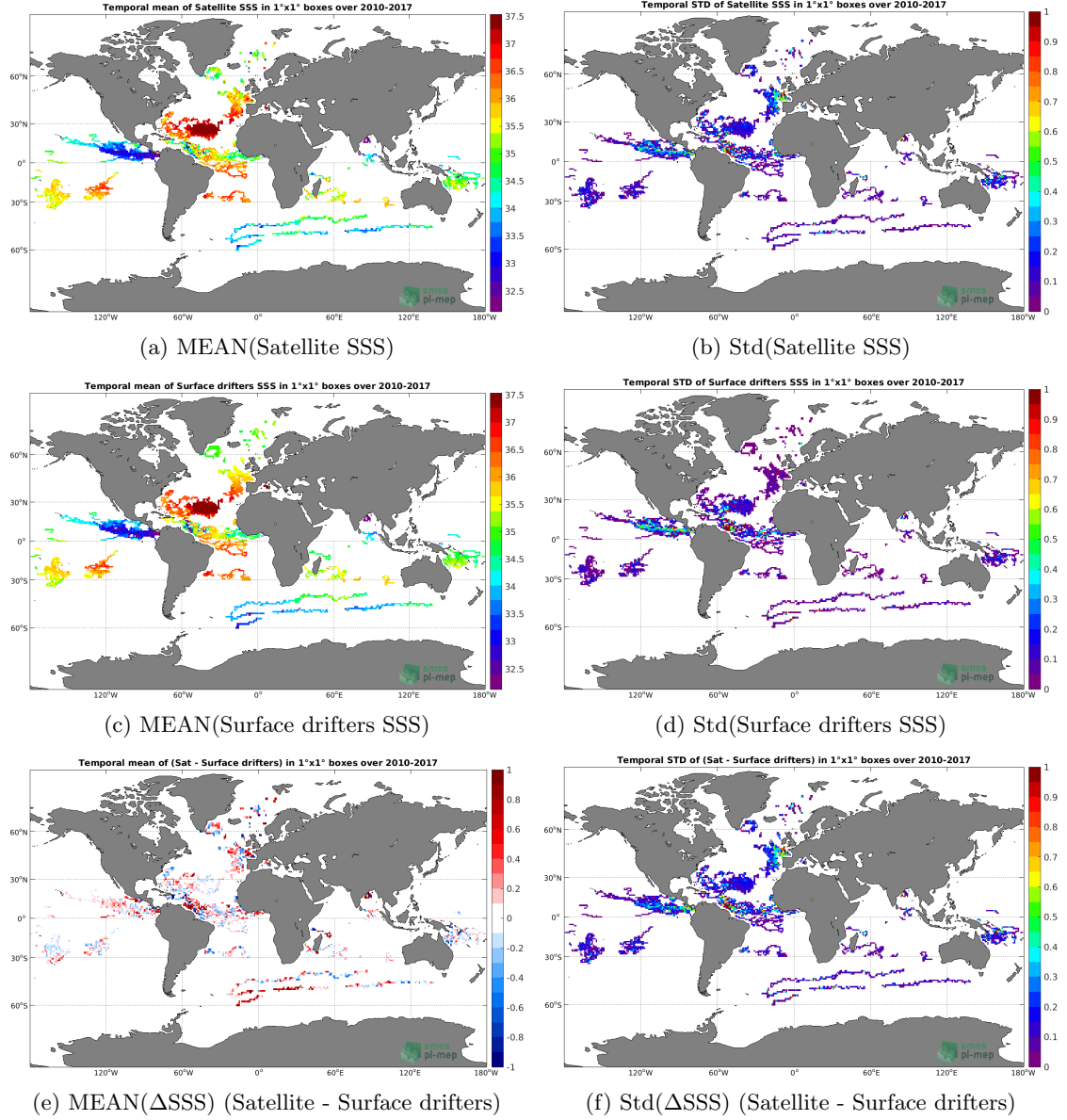
Figure 5: Temporal mean (left) and Std (right) of SSS from SMOS L4 v2 Weekly (CATDS-CECOS-IFREMER) (top), Surface drifters (middle), and of \Delta SSS (Satellite - Surface drifters). Only match-up pairs are used to generate these maps.
