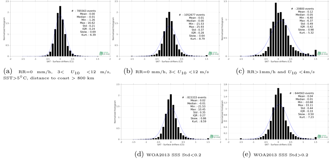
Figure 12: Normalized histogram of \Delta SSS (SMOS L4 v2 Weekly (CATDS-CECOS-IFREMER) - Surface drifters) for 5 different subdatasets corresponding to: RR=0 mm/h, 3 < U_{10} < 12 m/s, SST>5°C, distance to coast > 800 km (a), RR=0 mm/h, 3 < U_{10} < 12 m/s (b), RR>1mm/h and U_{10} < 4 m/s (c), WOA2013 SSS Std<0.2 (d), WOA2013 SSS Std>0.2 (e).
