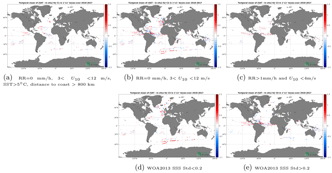
Figure 11: Temporal mean gridded over spatial boxes of size 1^\circ \times 1^\circ of \Delta SSS (SMOS L4 v2 Weekly (CATDS-CECOS-IFREMER) - Surface drifters) for 5 different subdatasets corresponding to:RR=0 mm/h, 3 < U_{10} < 12 m/s, SST>5°C, distance to coast > 800 km (a), RR=0 mm/h, 3 < U_{10} < 12 m/s (b), RR>1mm/h and U_{10} < 4 m/s (c), WOA2013 SSS Std<0.2 (d), WOA2013 SSS Std>0.2 (e).
