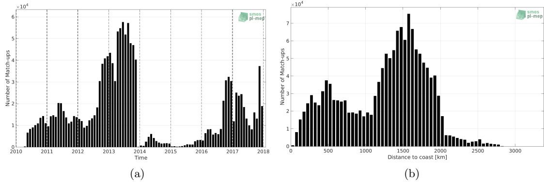
Figure 1: Number of match-ups between Surface drifters and SMOS L4 v2 Weekly (CATDS-CECOS-IFREMER) SSS as a function of time (a) and as function of the distance to coast (b) over the Global Ocean Pi-MEP region and for the full satellite product period.
