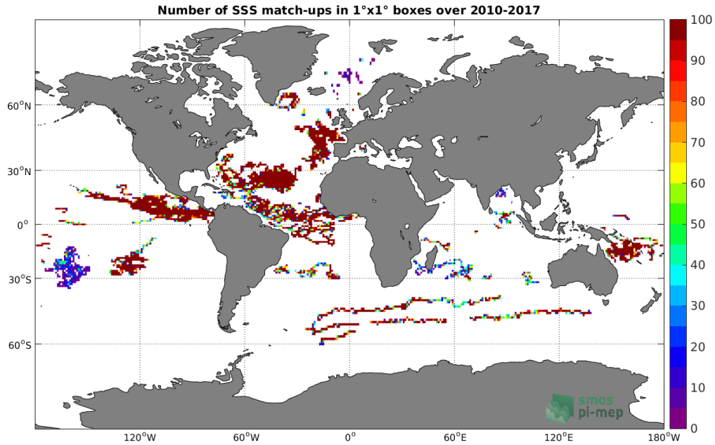
Figure 3: Number of SSS match-ups between Surface drifters SSS and the SMOS-L4-CATDS-CECOS-IFREMER-V2-WEEKLY-0.5DEG SSS product for the Global Ocean Pi-MEP region over 1°x1° boxes and for the full satellite product period.
