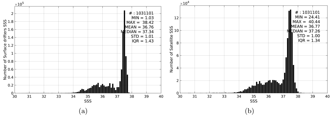
Figure 2: Histograms of SSS from Surface drifters (a) and SMOS-L4-CATDS-CECOS-IFREMER-V2-WEEKLY-0.5DEG (b) considering all match-up pairs per bins of 0.1 over the Global Ocean Pi-MEP region and for the full satellite product period.
