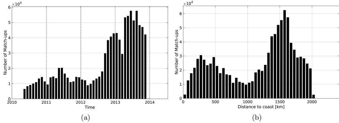
Figure 1: Number of match-ups between Surface drifters and SMOS-L4-CATDS-CECOS-IFREMER-V2-WEEKLY-0.5DEG SSS as a function of time (a) and as function of the distance to coast (b) over the Global Ocean Pi-MEP region and for the full satellite product period.
