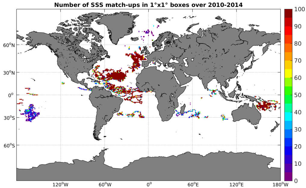
Figure 3: Number of SSS match-ups between Surface drifters SSS and the SMOS-L4-CATDS-CECOS-IFREMER-V2-WEEKLY-0.5DEG SSS product for the Global Ocean Pi-MEP region over 1°x1° boxes and for the full satellite product period.
