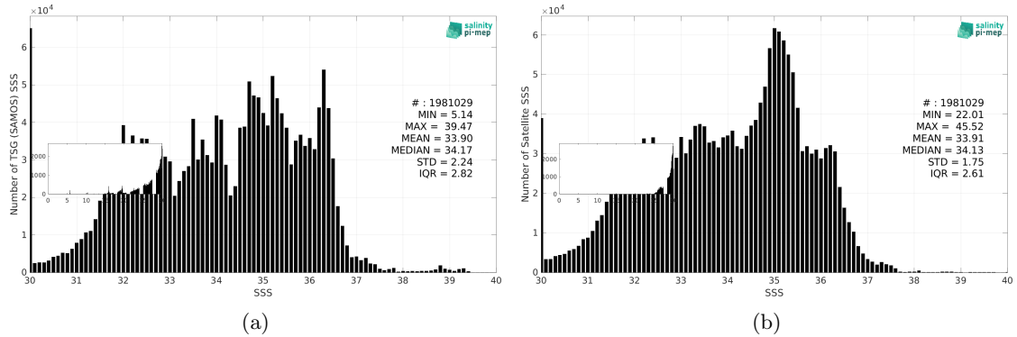
Figure 3: Histograms of SSS from TSG (SAMOS) (a) and SMOS SSS L4 v2 - Daily (BEC) (b) considering all match-up pairs per bins of 0.1 over the Global Ocean Pi-MEP region and for the full satellite product period.
