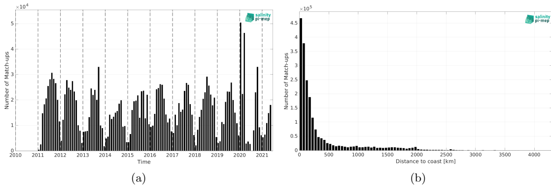
Figure 2: Number of match-ups between TSG (SAMOS) and SMOS SSS L4 v2 - Daily (BEC) SSS as a function of time (a) and as function of the distance to coast (b) over the Global Ocean Pi-MEP region and for the full satellite product period.
