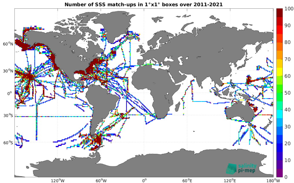
Figure 5: Number of SSS match-ups between TSG (SAMOS) SSS and the SMOS SSS L4 v2 - Daily (BEC) SSS product for the Global Ocean Pi-MEP region over 1^\circ \times 1^\circ boxes and for the full satellite product period.
