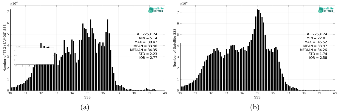
Figure 2: Histograms of SSS from TSG (SAMOS) (a) and SMOS SSS L4 v2 - Daily (BEC) (b) considering all match-up pairs per bins of 0.1 over the Global Ocean Pi-MEP region and for the full satellite product period.
