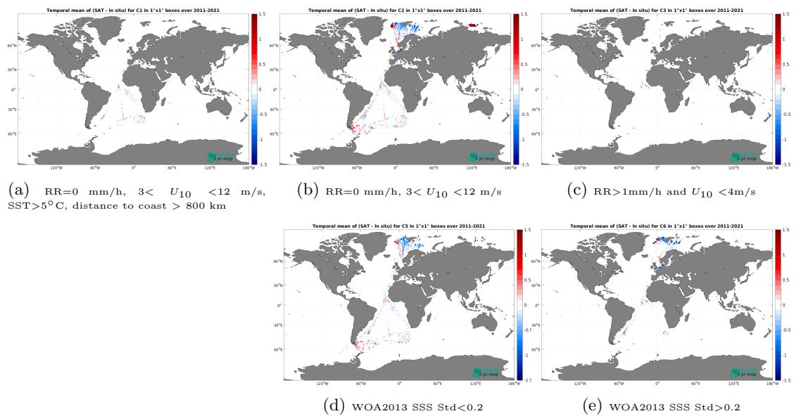
Figure 14: Temporal mean gridded over spatial boxes of size 1^\circ \times 1^\circ of \Delta\text{SSS} (SMOS SSS L4 v2 - Daily (BEC) - TSG (Polarstern)) for 5 different subdatasets corresponding to:RR=0 mm/h, 3 < U_{10} < 12 m/s, SST > 5^\circ\text{C} , distance to coast > 800 km (a), RR=0 mm/h, 3 < U_{10} < 12 m/s (b), RR > 1 mm/h and U_{10} < 4 m/s (c), WOA2013 SSS Std < 0.2 (d), WOA2013 SSS Std > 0.2 (e).
