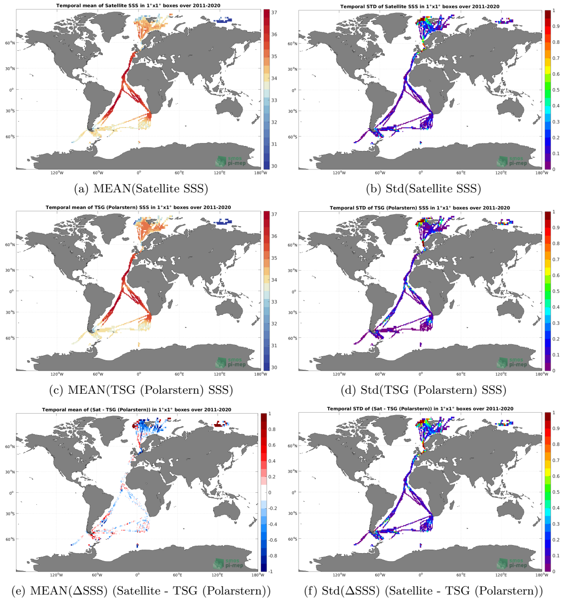
Figure 6: Temporal mean (left) and Std (right) of SSS from SMOS SSS L4 v2 - Daily (BEC) (top), TSG (Polarstern) (middle), and of \Delta SSS (Satellite - TSG (Polarstern)). Only match-up pairs are used to generate these maps.
