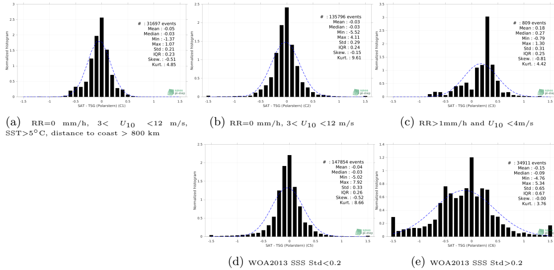
Figure 13: Normalized histogram of \Delta SSS (SMOS SSS L4 v2 - Daily (BEC) - TSG (Polarstern)) for 5 different subdatasets corresponding to: RR=0 mm/h, 3 < U_{10} < 12 m/s, SST>5°C, distance to coast > 800 km (a), RR=0 mm/h, 3 < U_{10} < 12 m/s (b), RR>1mm/h and U_{10} < 4 m/s (c), WOA2013 SSS Std<0.2 (d), WOA2013 SSS Std>0.2 (e).
