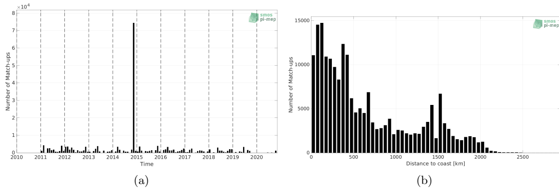
Figure 1: Number of match-ups between TSG (Polarstern) and SMOS SSS L4 v2 - Daily (BEC) SSS as a function of time (a) and as function of the distance to coast (b) over the Global Ocean Pi-MEP region and for the full satellite product period.
