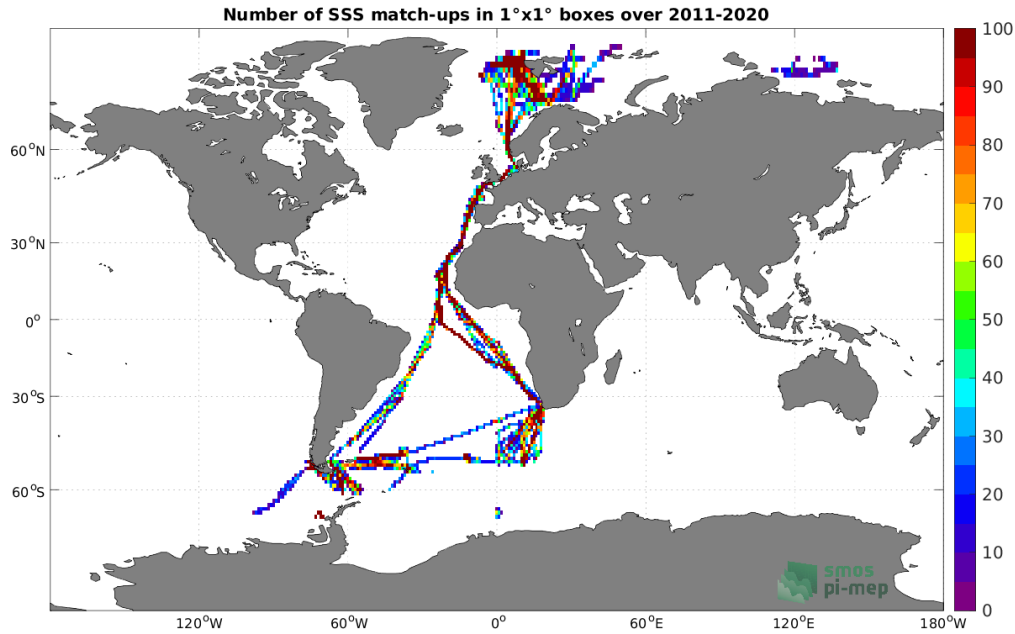
Figure 4: Number of SSS match-ups between TSG (Polarstern) SSS and the SMOS SSS L4 v2 - Daily (BEC) SSS product for the Global Ocean Pi-MEP region over 1^\circ \times 1^\circ boxes and for the full satellite product period.
