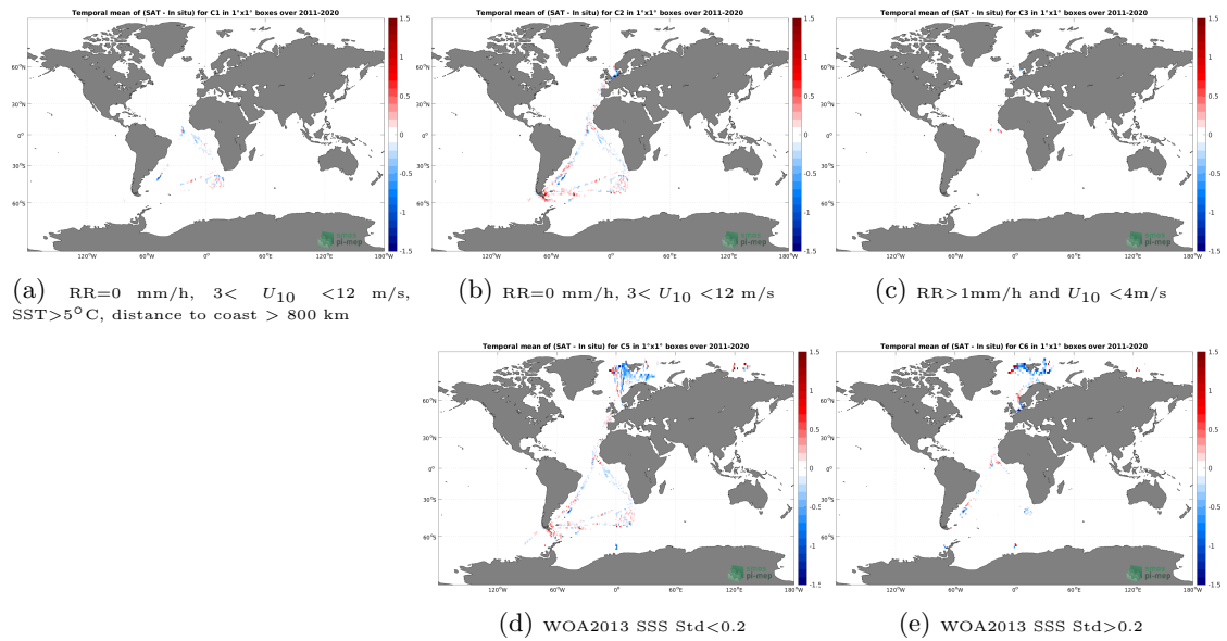
Figure 12: Temporal mean gridded over spatial boxes of size 1^\circ \times 1^\circ of \Delta SSS (SMOS SSS L4 v2 - Daily (BEC) - TSG (Polarstern)) for 5 different subdatasets corresponding to:RR=0 mm/h, 3 < U_{10} < 12 m/s, SST >5^\circ C, distance to coast > 800 km (a), RR=0 mm/h, 3 < U_{10} < 12 m/s (b), RR >1 mm/h and U_{10} < 4 m/s (c), WOA2013 SSS Std <0.2 (d), WOA2013 SSS Std >0.2 (e).
