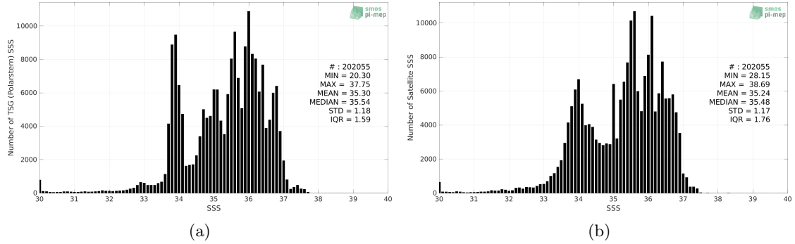
Figure 2: Histograms of SSS from TSG (Polarstern) (a) and SMOS SSS L4 v2 - Daily (BEC) (b) considering all match-up pairs per bins of 0.1 over the Global Ocean Pi-MEP region and for the full satellite product period.
