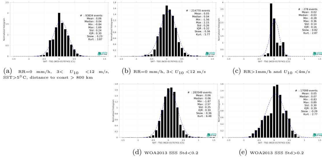
Figure 15: Normalized histogram of \Delta\text{SSS} (SMOS SSS L4 v2 - Daily (BEC) - TSG (NCEI-0170743)) for 5 different subdatasets corresponding to: RR=0 mm/h, 3 < U_{10} < 12 m/s, SST>5°C, distance to coast > 800 km (a), RR=0 mm/h, 3 < U_{10} < 12 m/s (b), RR>1mm/h and U_{10} < 4 m/s (c), WOA2013 SSS Std<0.2 (d), WOA2013 SSS Std>0.2 (e).
