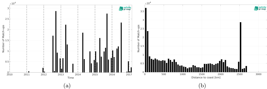
Figure 2: Number of match-ups between TSG (NCEI-0170743) and SMOS SSS L4 v2 - Daily (BEC) SSS as a function of time (a) and as function of the distance to coast (b) over the Global Ocean Pi-MEP region and for the full satellite product period.
