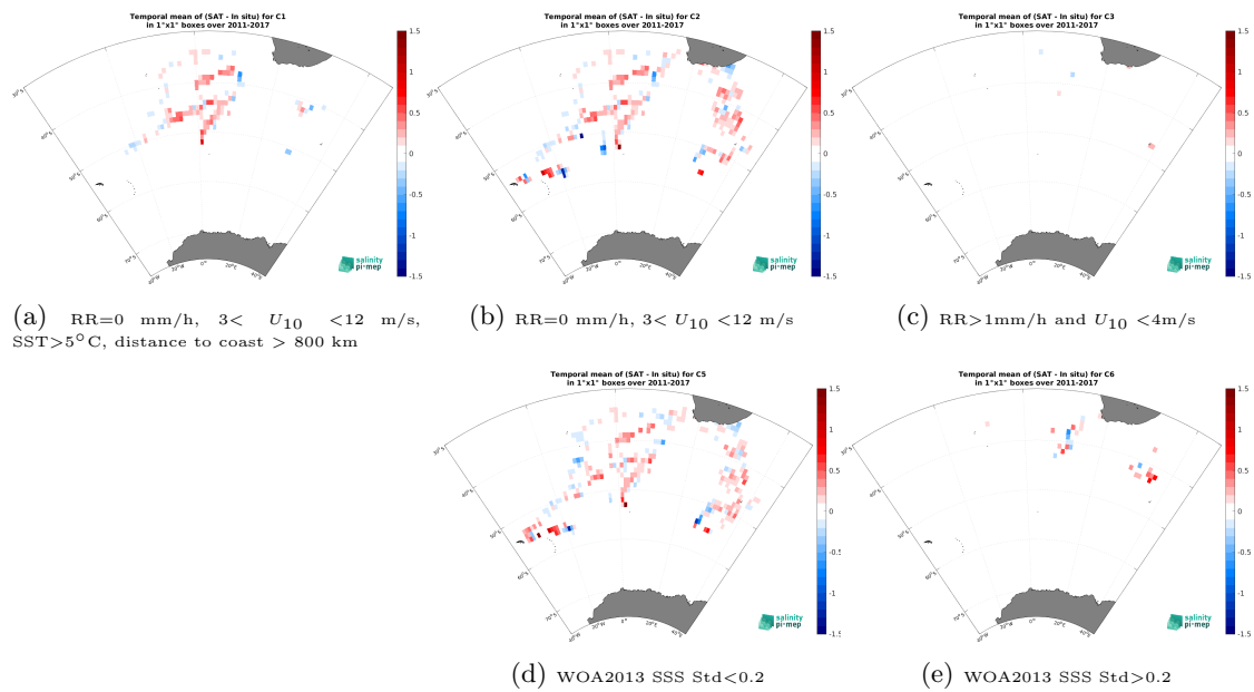
Figure 14: Temporal mean gridded over spatial boxes of size 1^\circ \times 1^\circ of \Delta SSS (SMOS SSS L4 v2 - Daily (BEC) - TSG (NCEI-0170743)) for 5 different subdatasets corresponding to:RR=0 mm/h, 3 < U_{10} < 12 m/s, SST > 5^\circ\text{C} , distance to coast > 800 km (a), RR=0 mm/h, 3 < U_{10} < 12 m/s (b), RR > 1 mm/h and U_{10} < 4 m/s (c), WOA2013 SSS Std < 0.2 (d), WOA2013 SSS Std > 0.2 (e).
