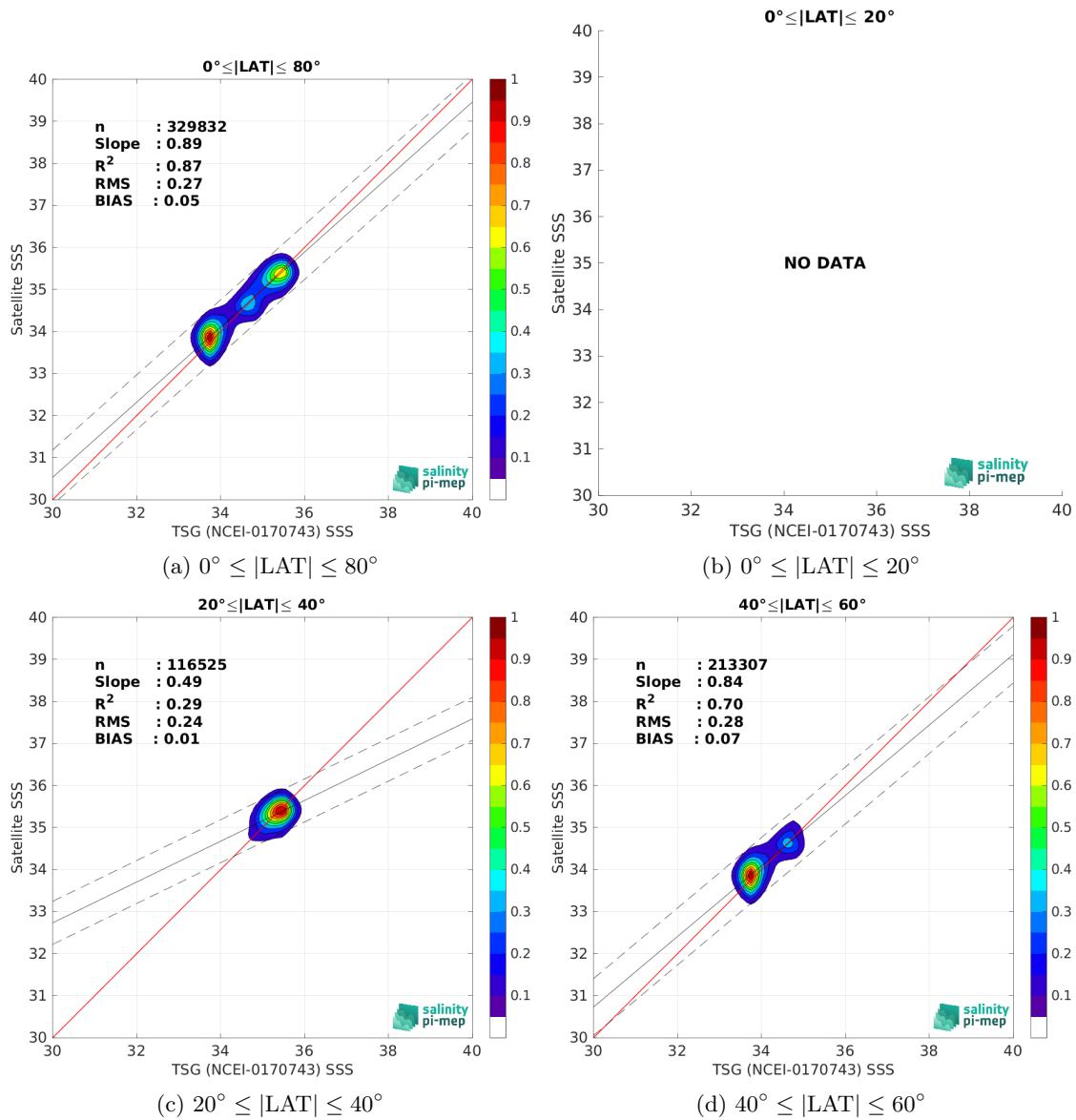
Figure 10: Contour maps of the concentration of SMOS SSS L4 v2 - Daily (BEC) SSS (y-axis) versus TSG (NCEI-0170743) SSS (x-axis) at match-up pairs for different latitude bands. For each plot, the red line shows x=y . The black thin and dashed lines indicate a linear fit through the data cloud and the \pm 95\% confidence levels, respectively. The number match-up pairs n , the slope and R^2 coefficient of the linear fit, the root mean square (RMS) and the mean bias between satellite and in situ data are indicated for each latitude band in each plots.
