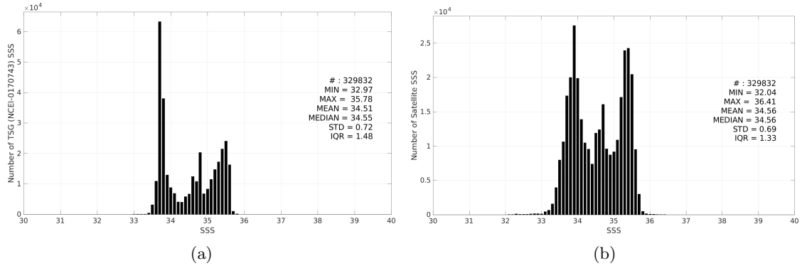
Figure 3: Histograms of SSS from TSG (NCEI-0170743) (a) and SMOS SSS L4 v2 - Daily (BEC) (b) considering all match-up pairs per bins of 0.1 over the Global Ocean Pi-MEP region and for the full satellite product period.
