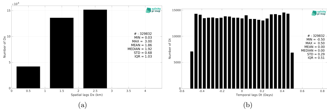
Figure 6: Histograms of the spatial (a) and temporal (b) lags between the location/time of the TSG (NCEI-0170743) measurement and the date of the corresponding SMOS SSS L4 v2 - Daily (BEC) SSS pixel.
