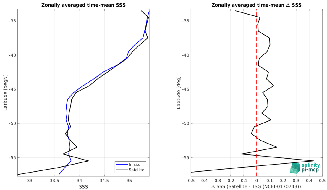
Figure 9: Left panel: Zonal mean SSS from SMOS SSS L4 v2 - Daily (BEC) satellite product (black) and from TSG (NCEI-0170743) (blue). Right panel: Zonal mean of \Delta SSS (Satellite - TSG (NCEI-0170743)) for all the collected Pi-MEP match-up pairs estimated over the full satellite product period.
