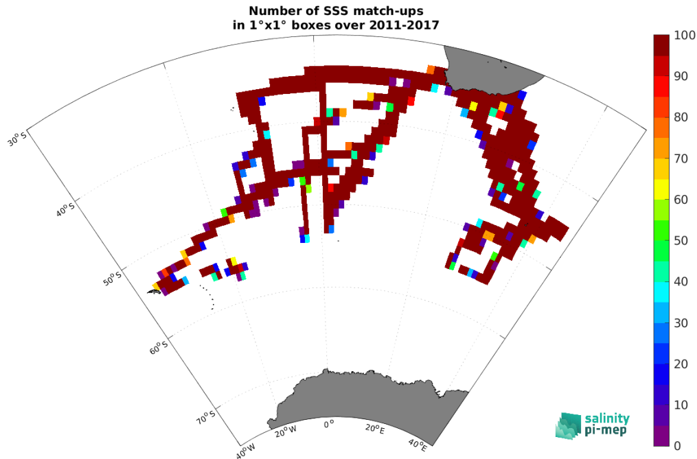
Figure 5: Number of SSS match-ups between TSG (NCEI-0170743) SSS and the SMOS SSS L4 v2 - Daily (BEC) SSS product for the Global Ocean Pi-MEP region over 1^\circ \times 1^\circ boxes and for the full satellite product period.
