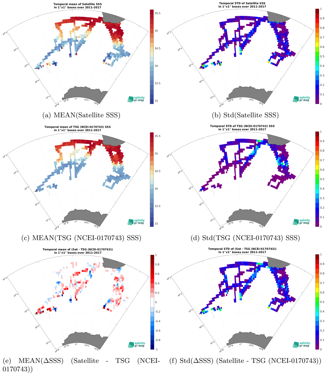
Figure 7: Temporal mean (left) and Std (right) of SSS from SMOS SSS L4 v2 - Daily (BEC) (top), TSG (NCEI-0170743) (middle), and of \Delta SSS (Satellite - TSG (NCEI-0170743)). Only match-up pairs are used to generate these maps.
