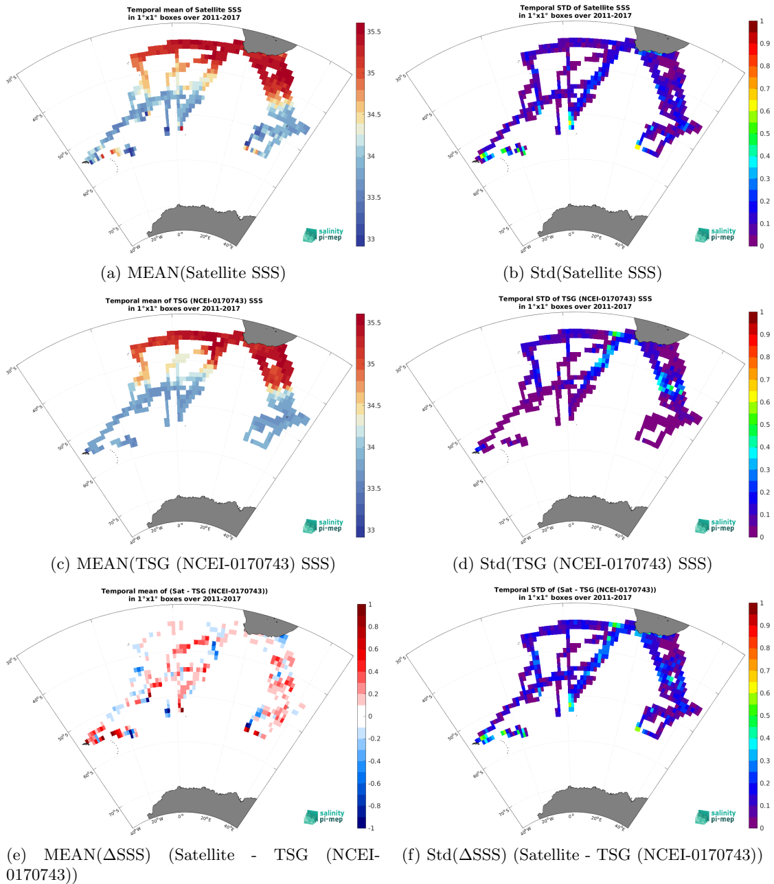
Figure 6: Temporal mean (left) and Std (right) of SSS from SMOS SSS L4 v2 - Daily (BEC) (top), TSG (NCEI-0170743) (middle), and of \Delta SSS (Satellite - TSG (NCEI-0170743)). Only match-up pairs are used to generate these maps.
