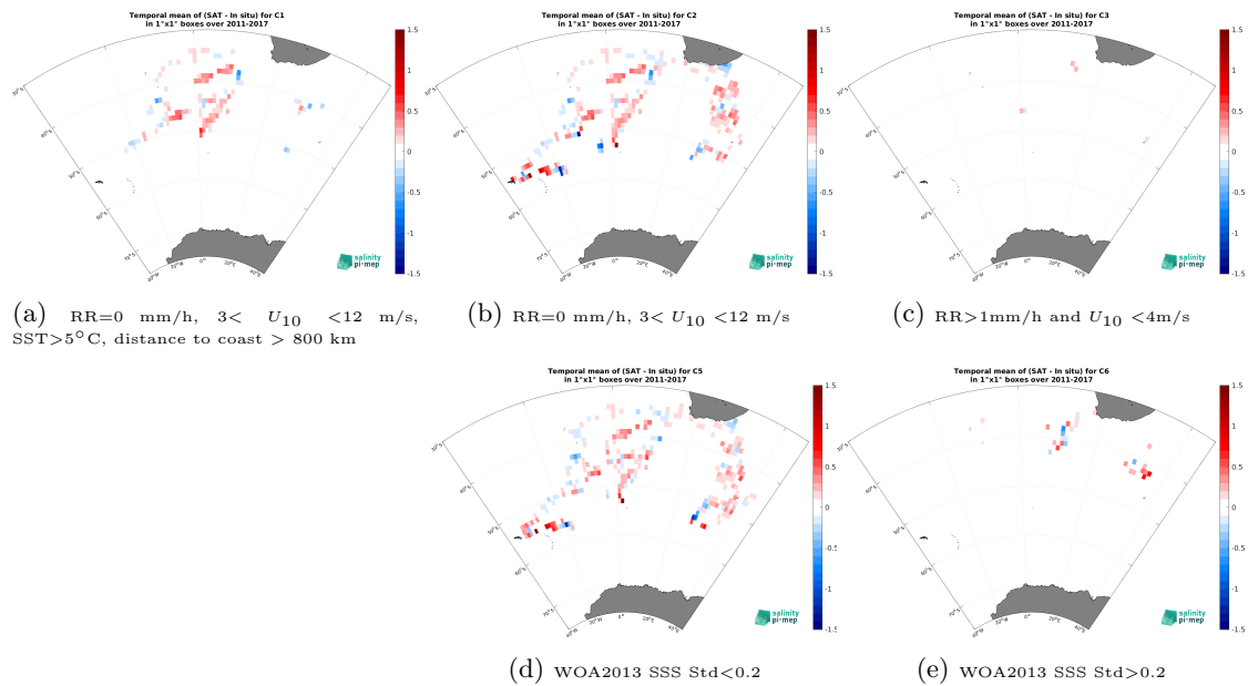
Figure 12: Temporal mean gridded over spatial boxes of size 1^\circ \times 1^\circ of \Delta\text{SSS} (SMOS SSS L4 v2 - Daily (BEC) - TSG (NCEI-0170743)) for 5 different subdatasets corresponding to:RR=0 mm/h, 3 < U_{10} < 12 m/s, SST >5^\circ\text{C} , distance to coast > 800 km (a), RR=0 mm/h, 3 < U_{10} < 12 m/s (b), RR >1 mm/h and U_{10} < 4 m/s (c), WOA2013 SSS Std <0.2 (d), WOA2013 SSS Std >0.2 (e).
