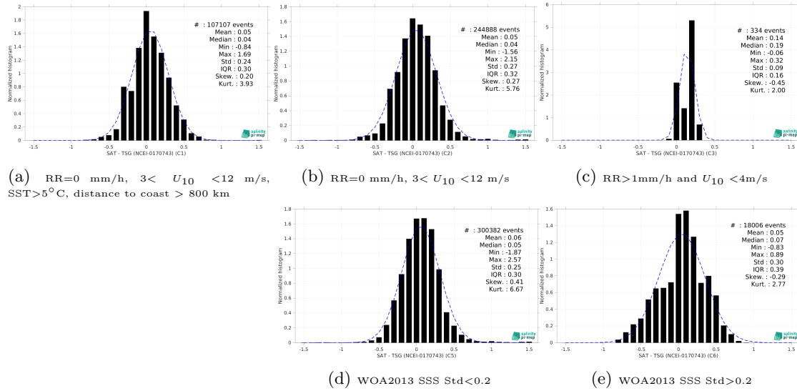
Figure 13: Normalized histogram of \Delta\text{SSS} (SMOS SSS L4 v2 - Daily (BEC) - TSG (NCEI-0170743)) for 5 different subdatasets corresponding to: RR=0 mm/h, 3 < U_{10} < 12 m/s, SST>5°C, distance to coast > 800 km (a), RR=0 mm/h, 3 < U_{10} < 12 m/s (b), RR>1mm/h and U_{10} < 4 m/s (c), WOA2013 SSS Std<0.2 (d), WOA2013 SSS Std>0.2 (e).
