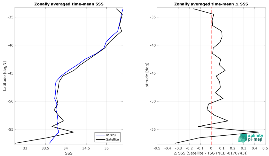
Figure 8: Left panel: Zonal mean SSS from SMOS SSS L4 v2 - Daily (BEC) satellite product (black) and from TSG (NCEI-0170743) (blue). Right panel: Zonal mean of \Delta SSS (Satellite - TSG (NCEI-0170743)) for all the collected Pi-MEP match-up pairs estimated over the full satellite product period.
