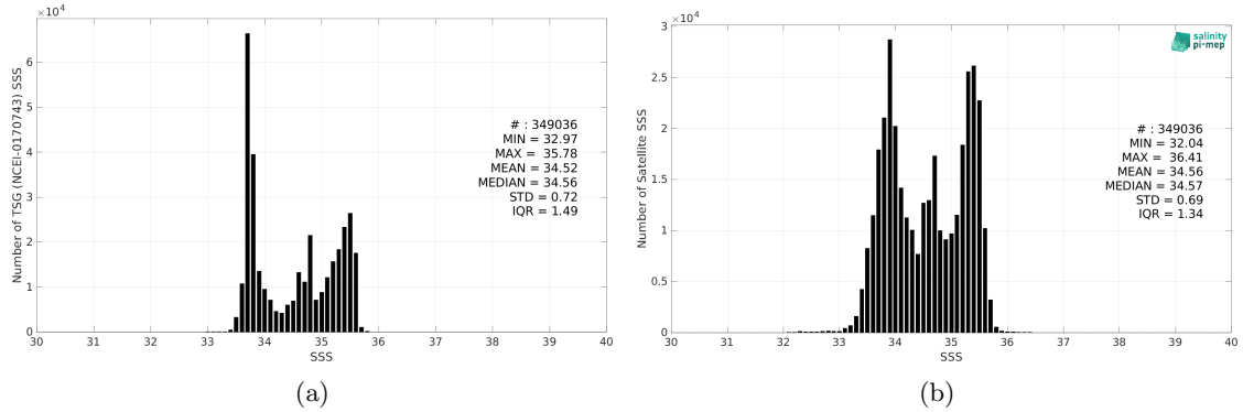
Figure 2: Histograms of SSS from TSG (NCEI-0170743) (a) and SMOS SSS L4 v2 - Daily (BEC) (b) considering all match-up pairs per bins of 0.1 over the Global Ocean Pi-MEP region and for the full satellite product period.
