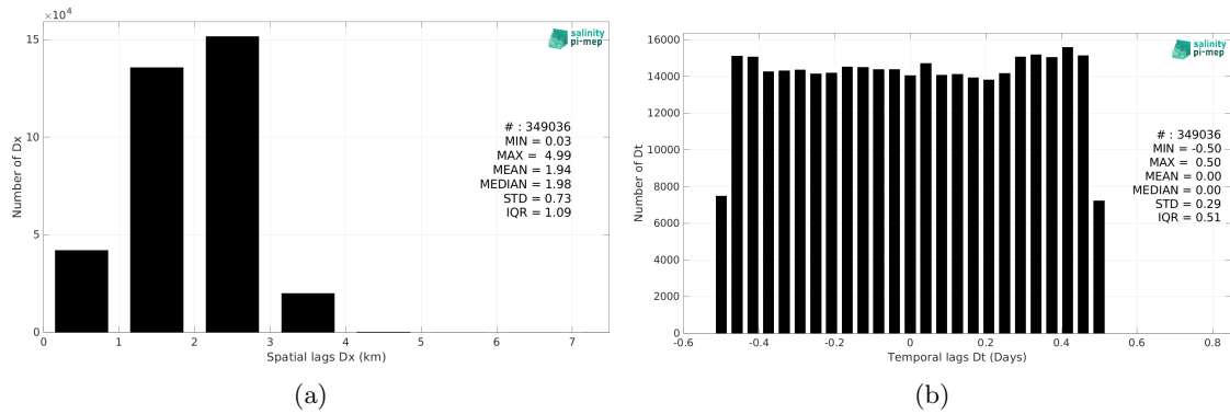
Figure 5: Histograms of the spatial (a) and temporal (b) lags between the location/time of the TSG (NCEI-0170743) measurement and the date of the corresponding SMOS SSS L4 v2 - Daily (BEC) SSS pixel.
