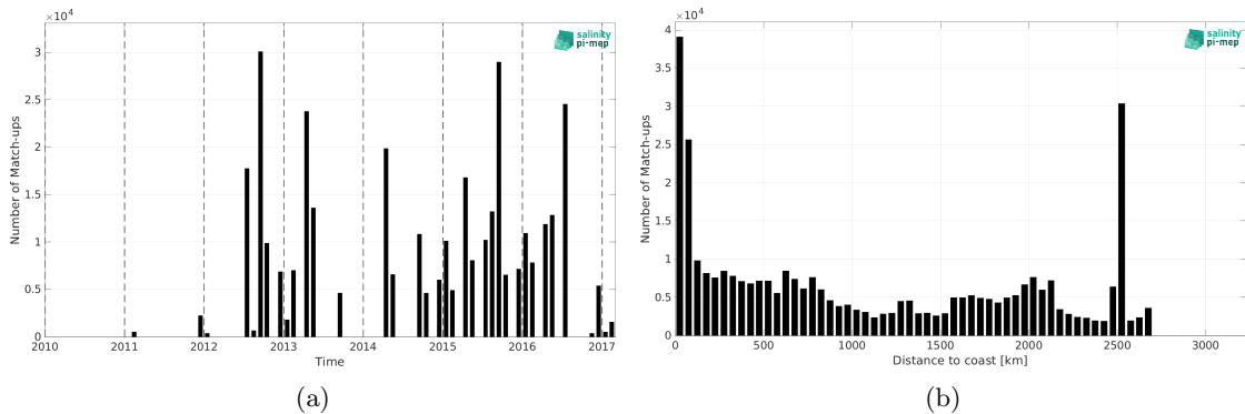
Figure 1: Number of match-ups between TSG (NCEI-0170743) and SMOS SSS L4 v2 - Daily (BEC) SSS as a function of time (a) and as function of the distance to coast (b) over the Global Ocean Pi-MEP region and for the full satellite product period.
