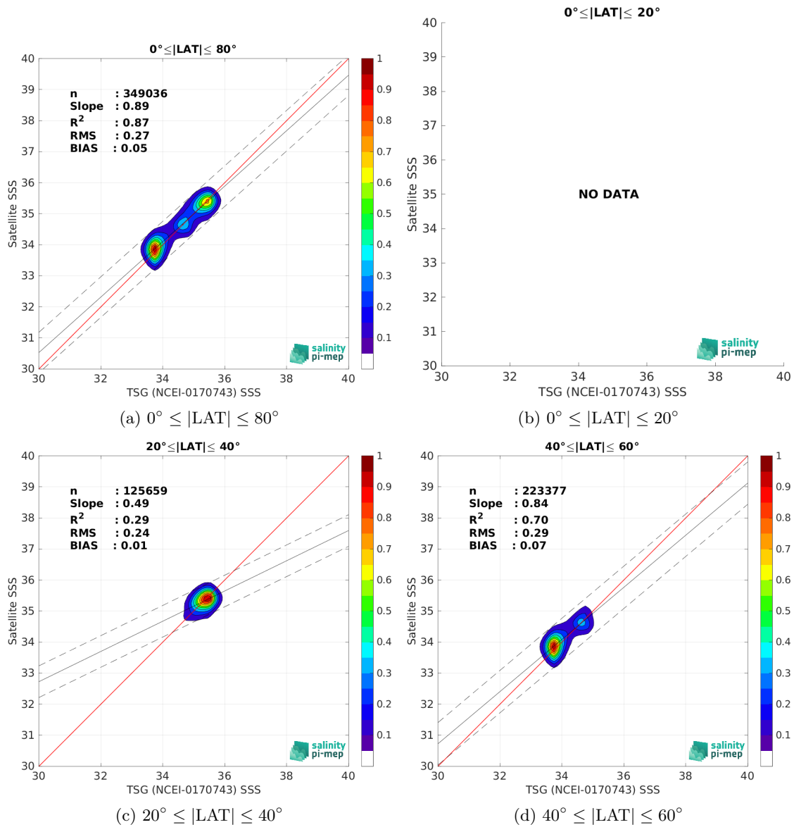
Figure 9: Contour maps of the concentration of SMOS SSS L4 v2 - Daily (BEC) SSS (y-axis) versus TSG (NCEI-0170743) SSS (x-axis) at match-up pairs for different latitude bands. For each plot, the red line shows x=y . The black thin and dashed lines indicate a linear fit through the data cloud and the \pm 95\% confidence levels, respectively. The number match-up pairs n , the slope and R^2 coefficient of the linear fit, the root mean square (RMS) and the mean bias between satellite and in situ data are indicated for each latitude band in each plots.
