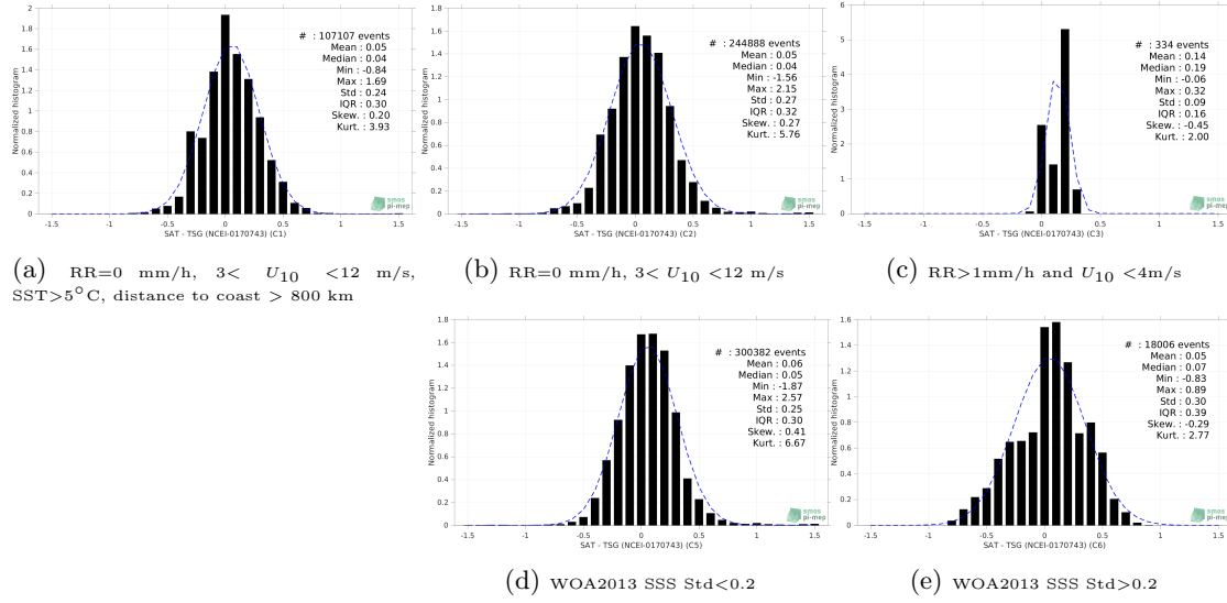
Figure 13: Normalized histogram of \Delta SSS (SMOS SSS L4 v2 - Daily (BEC) - TSG (NCEI-0170743)) for 5 different subdatasets corresponding to: RR=0 mm/h, 3 < U_{10} < 12 m/s, SST > 5°C, distance to coast > 800 km (a), RR=0 mm/h, 3 < U_{10} < 12 m/s (b), RR > 1mm/h and U_{10} < 4 m/s (c), WOA2013 SSS Std < 0.2 (d), WOA2013 SSS Std > 0.2 (e).
