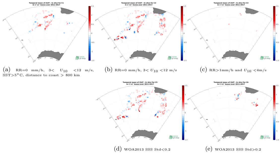
Figure 12: Temporal mean gridded over spatial boxes of size 1^\circ \times 1^\circ of \Delta SSS (SMOS SSS L4 v2 - Daily (BEC) - TSG (NCEI-0170743)) for 5 different subdatasets corresponding to:RR=0 mm/h, 3 < U_{10} < 12 m/s, SST >5^\circ C, distance to coast > 800 km (a), RR=0 mm/h, 3 < U_{10} < 12 m/s (b), RR >1 mm/h and U_{10} < 4 m/s (c), WOA2013 SSS Std <0.2 (d), WOA2013 SSS Std >0.2 (e).
