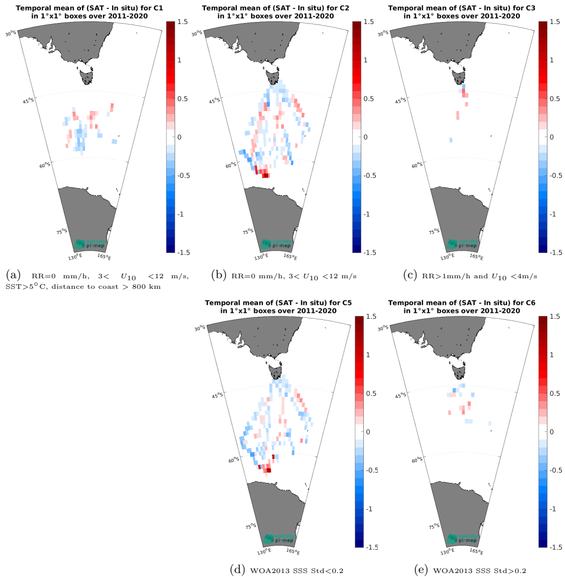
Figure 14: Temporal mean gridded over spatial boxes of size 1^\circ \times 1^\circ of \Delta SSS (SMOS SSS L4 v2 - Daily (BEC) - TSG (LEGOS-Survostral)) for 5 different subdatasets corresponding to: RR=0 mm/h, 3 < U_{10} < 12 m/s, SST>5°C, distance to coast > 800 km (a), RR=0 mm/h, 3 < U_{10} < 12 m/s (b), RR>1mm/h and U_{10} < 4 m/s (c), WOA2013 SSS Std<0.2 (d), WOA2013 SSS Std>0.2 (e).
