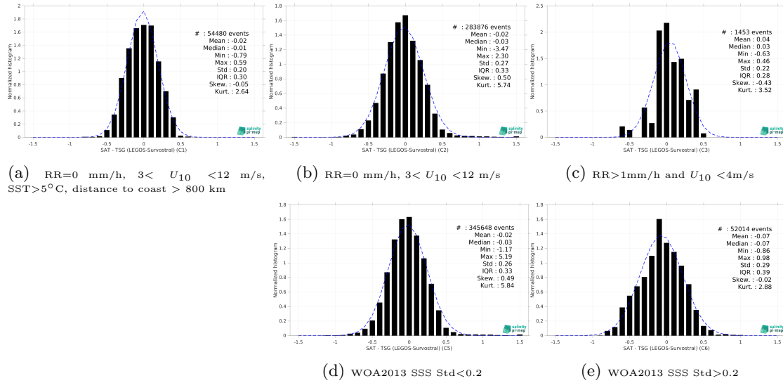
Figure 15: Normalized histogram of \Delta SSS (SMOS SSS L4 v2 - Daily (BEC) - TSG (LEGOS-Survostral)) for 5 different subdatasets corresponding to: RR=0 mm/h, 3 < U_{10} < 12 m/s, SST > 5°C, distance to coast > 800 km (a), RR=0 mm/h, 3 < U_{10} < 12 m/s (b), RR > 1mm/h and U_{10} < 4 m/s (c), WOA2013 SSS Std < 0.2 (d), WOA2013 SSS Std > 0.2 (e).
