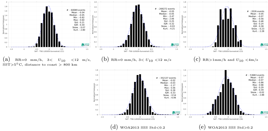
Figure 13: Normalized histogram of \Delta SSS (SMOS SSS L4 v2 - Daily (BEC) - TSG (LEGOS-Survostral)) for 5 different subdatasets corresponding to: RR=0 mm/h, 3 < U_{10} < 12 m/s, SST > 5°C, distance to coast > 800 km (a), RR=0 mm/h, 3 < U_{10} < 12 m/s (b), RR > 1mm/h and U_{10} < 4 m/s (c), WOA2013 SSS Std < 0.2 (d), WOA2013 SSS Std > 0.2 (e).
