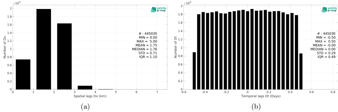
Figure 5: Histograms of the spatial (a) and temporal (b) lags between the location/time of the TSG (LEGOS-Survostral) measurement and the date of the corresponding SMOS SSS L4 v2 - Daily (BEC) SSS pixel.
