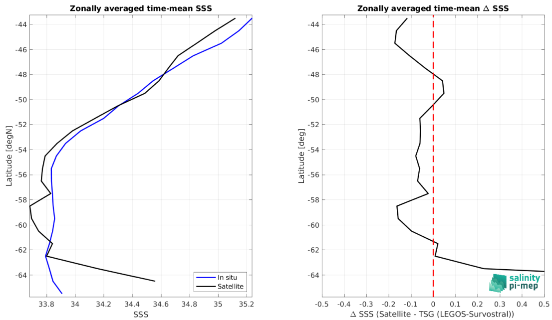
Figure 8: Left panel: Zonal mean SSS from SMOS SSS L4 v2 - Daily (BEC) satellite product (black) and from TSG (LEGOS-Survostral) (blue). Right panel: Zonal mean of \Delta SSS (Satellite - TSG (LEGOS-Survostral)) for all the collected Pi-MEP match-up pairs estimated over the full satellite product period.
