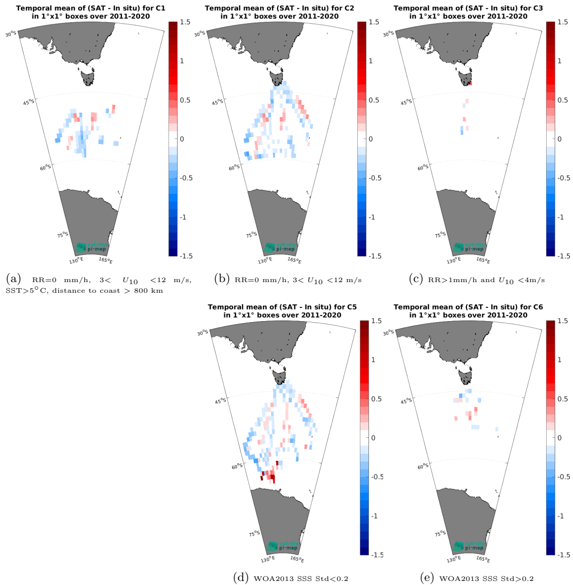
Figure 12: Temporal mean gridded over spatial boxes of size 1^\circ \times 1^\circ of \Delta SSS (SMOS SSS L4 v2 - Daily (BEC) - TSG (LEGOS-Survostral)) for 5 different subdatasets corresponding to:RR=0 mm/h, 3 < U_{10} < 12 m/s, SST>5°C, distance to coast > 800 km (a), RR=0 mm/h, 3 < U_{10} < 12 m/s (b), RR>1mm/h and U_{10} < 4 m/s (c), WOA2013 SSS Std<0.2 (d), WOA2013 SSS Std>0.2 (e).
