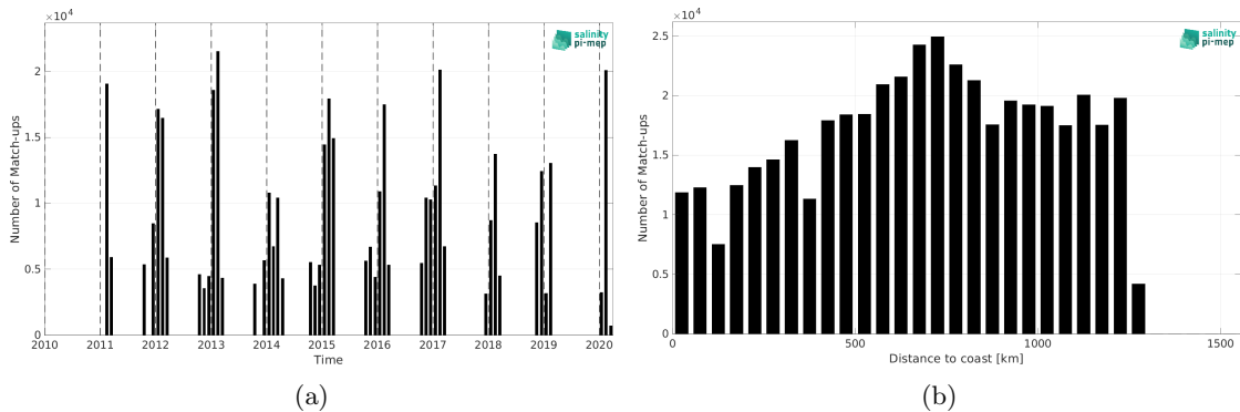
Figure 1: Number of match-ups between TSG (LEGOS-Survostral) and SMOS SSS L4 v2 - Daily (BEC) SSS as a function of time (a) and as function of the distance to coast (b) over the Global Ocean Pi-MEP region and for the full satellite product period.
