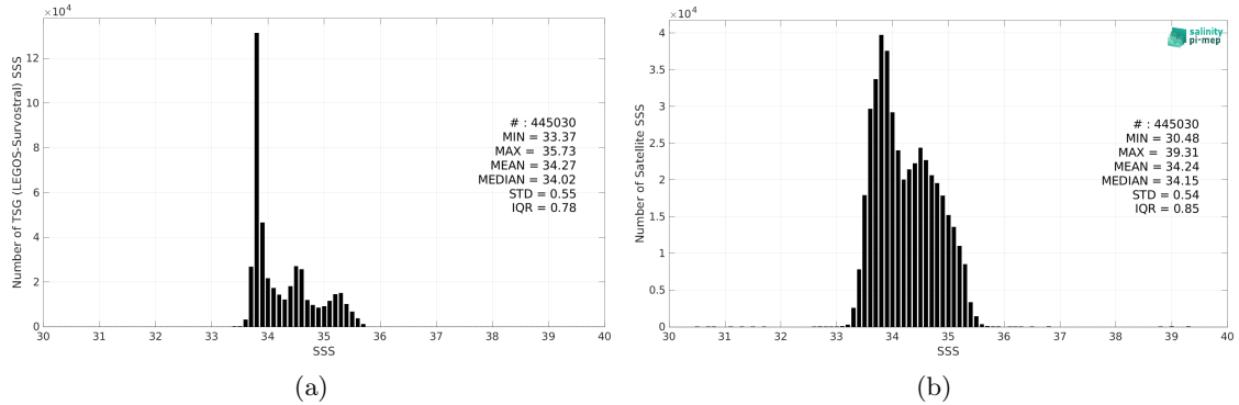
Figure 2: Histograms of SSS from TSG (LEGOS-Survostral) (a) and SMOS SSS L4 v2 - Daily (BEC) (b) considering all match-up pairs per bins of 0.1 over the Global Ocean Pi-MEP region and for the full satellite product period.
