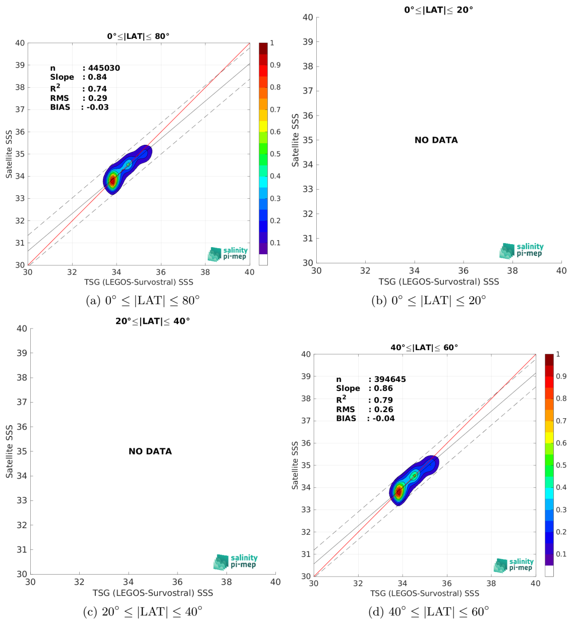
Figure 9: Contour maps of the concentration of SMOS SSS L4 v2 - Daily (BEC) SSS (y-axis) versus TSG (LEGOS-Survostral) SSS (x-axis) at match-up pairs for different latitude bands. For each plot, the red line shows x=y . The black thin and dashed lines indicate a linear fit through the data cloud and the \pm 95\% confidence levels, respectively. The number match-up pairs n , the slope and R^2 coefficient of the linear fit, the root mean square (RMS) and the mean bias between satellite and in situ data are indicated for each latitude band in each plots.
