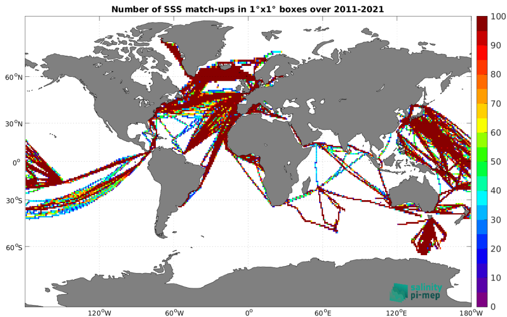
Figure 5: Number of SSS match-ups between TSG (LEGOS-DM) SSS and the SMOS SSS L4 v2 - Daily (BEC) SSS product for the Global Ocean Pi-MEP region over 1^\circ \times 1^\circ boxes and for the full satellite product period.
