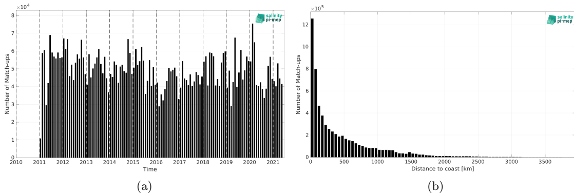
Figure 2: Number of match-ups between TSG (LEGOS-DM) and SMOS SSS L4 v2 - Daily (BEC) SSS as a function of time (a) and as function of the distance to coast (b) over the Global Ocean Pi-MEP region and for the full satellite product period.
