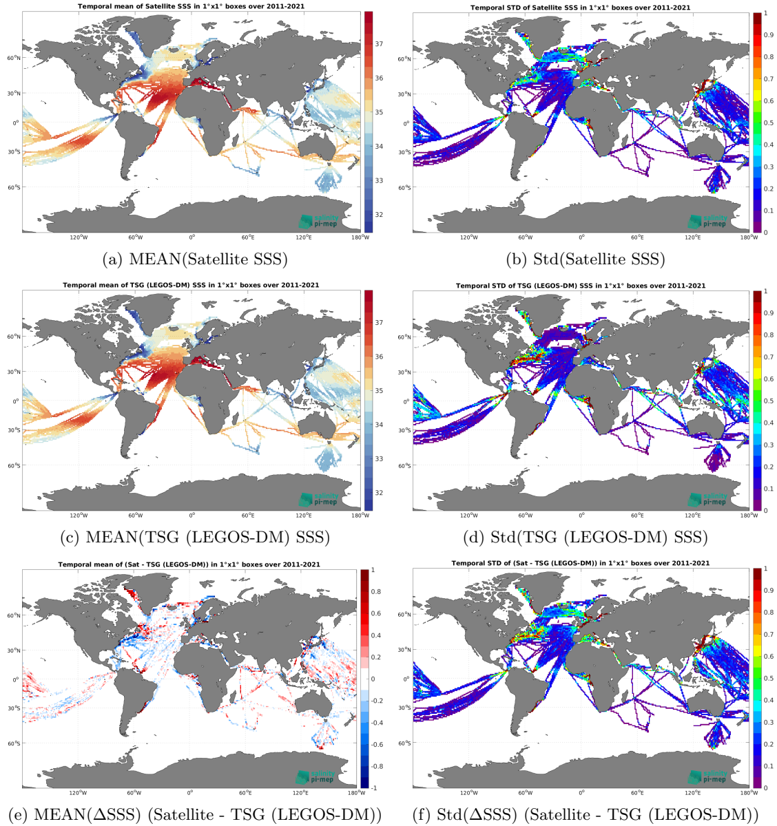
Figure 7: Temporal mean (left) and Std (right) of SSS from SMOS SSS L4 v2 - Daily (BEC) (top), TSG (LEGOS-DM) (middle), and of \Delta SSS (Satellite - TSG (LEGOS-DM)). Only match-pairs are used to generate these maps.
