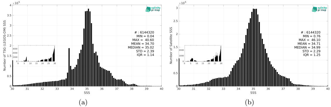
Figure 3: Histograms of SSS from TSG (LEGOS-DM) (a) and SMOS SSS L4 v2 - Daily (BEC) (b) considering all match-up pairs per bins of 0.1 over the Global Ocean Pi-MEP region and for the full satellite product period.
