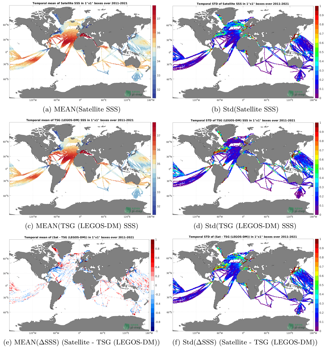
Figure 6: Temporal mean (left) and Std (right) of SSS from SMOS SSS L4 v2 - Daily (BEC) (top), TSG (LEGOS-DM) (middle), and of \Delta SSS (Satellite - TSG (LEGOS-DM)). Only match-pairs are used to generate these maps.
