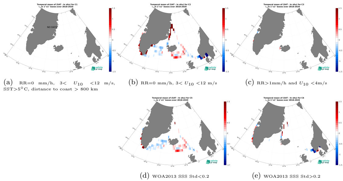
Figure 14: Temporal mean gridded over spatial boxes of size 1^\circ \times 1^\circ of \Delta\text{SSS} (SMOS SSS L4 v2 - Daily (BEC) - TSG (Lauge-Koch)) for 5 different subdatasets corresponding to:RR=0 mm/h, 3 < U_{10} < 12 m/s, SST > 5^\circ\text{C} , distance to coast > 800 km (a), RR=0 mm/h, 3 < U_{10} < 12 m/s (b), RR > 1 mm/h and U_{10} < 4 m/s (c), WOA2013 SSS Std < 0.2 (d), WOA2013 SSS Std > 0.2 (e).
