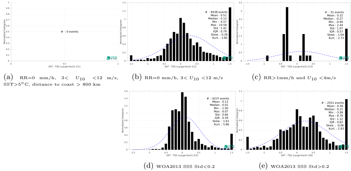
Figure 15: Normalized histogram of \Delta SSS (SMOS SSS L4 v2 - Daily (BEC) - TSG (Lauge-Koch)) for 5 different subdatasets corresponding to: RR=0 mm/h, 3 < U_{10} < 12 m/s, SST > 5°C, distance to coast > 800 km (a), RR=0 mm/h, 3 < U_{10} < 12 m/s (b), RR > 1mm/h and U_{10} < 4 m/s (c), WOA2013 SSS Std < 0.2 (d), WOA2013 SSS Std > 0.2 (e).
