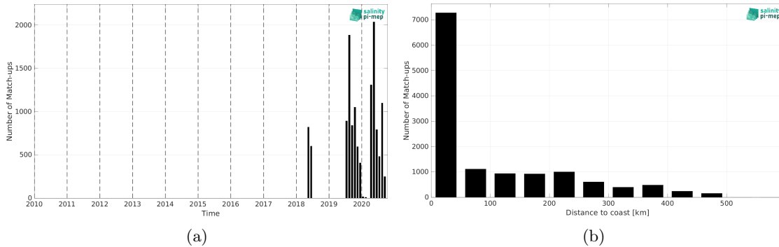
Figure 2: Number of match-ups between TSG (Lauge-Koch) and SMOS SSS L4 v2 - Daily (BEC) SSS as a function of time (a) and as function of the distance to coast (b) over the Global Ocean Pi-MEP region and for the full satellite product period.
