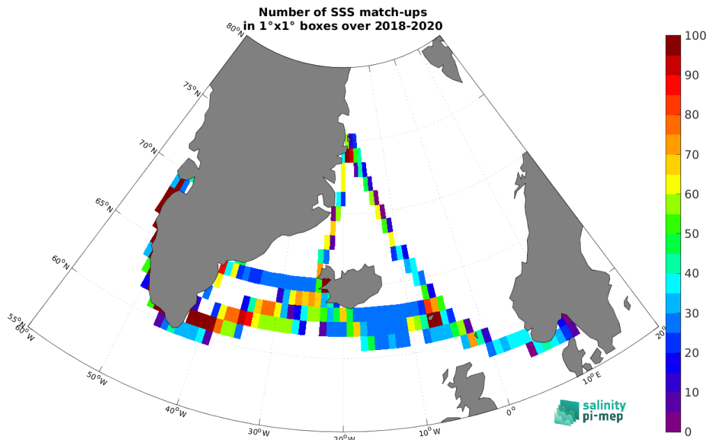
Figure 5: Number of SSS match-ups between TSG (Lauge-Koch) SSS and the SMOS SSS L4 v2 - Daily (BEC) SSS product for the Global Ocean Pi-MEP region over 1^\circ \times 1^\circ boxes and for the full satellite product period.
