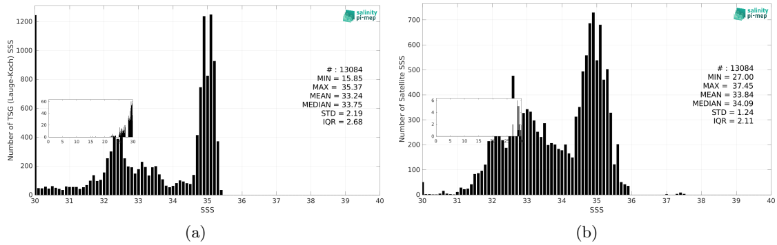
Figure 3: Histograms of SSS from TSG (Lauge-Koch) (a) and SMOS SSS L4 v2 - Daily (BEC) (b) considering all match-up pairs per bins of 0.1 over the Global Ocean Pi-MEP region and for the full satellite product period.
