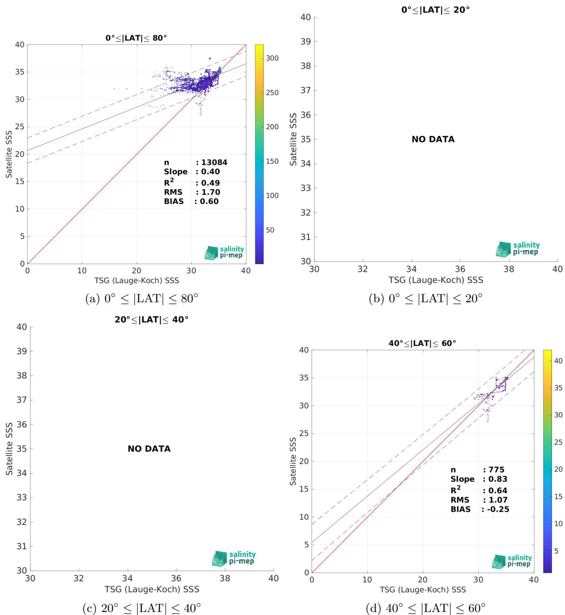
Figure 10: Contour maps of the concentration of SMOS SSS L4 v2 - Daily (BEC) SSS (y-axis) versus TSG (Lauge-Koch) SSS (x-axis) at match-up pairs for different latitude bands. For each plot, the red line shows x=y . The black thin and dashed lines indicate a linear fit through the data cloud and the \pm 95\% confidence levels, respectively. The number match-up pairs n , the slope and R^2 coefficient of the linear fit, the root mean square (RMS) and the mean bias between satellite and in situ data are indicated for each latitude band in each plots.
