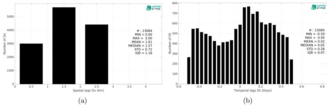
Figure 6: Histograms of the spatial (a) and temporal (b) lags between the location/time of the TSG (Lauge-Koch) measurement and the date of the corresponding SMOS SSS L4 v2 - Daily (BEC) SSS pixel.
