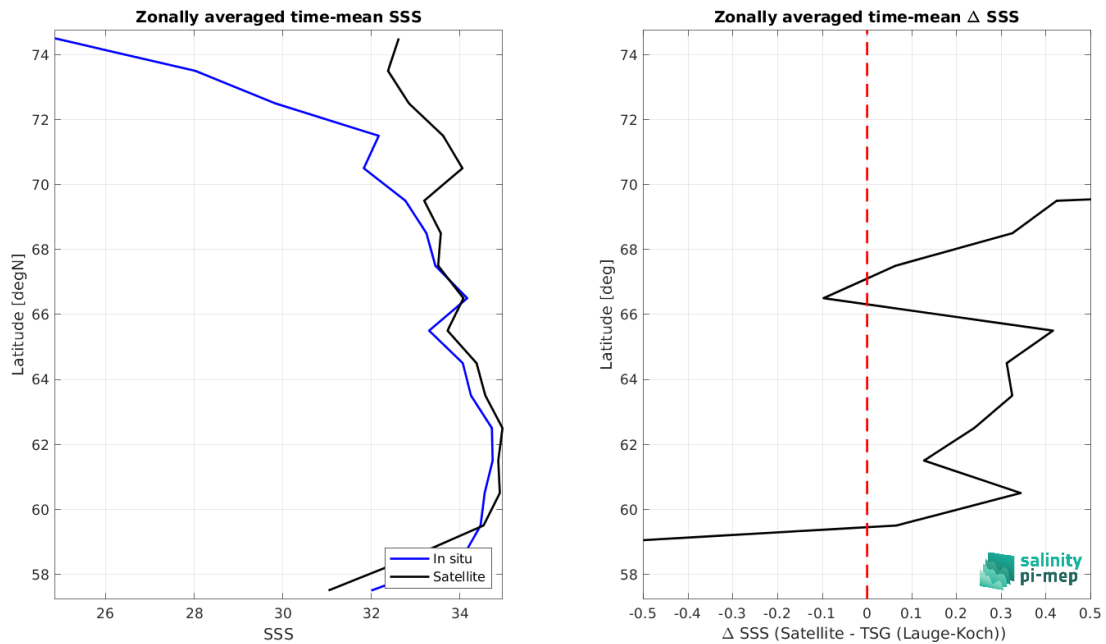
Figure 9: Left panel: Zonal mean SSS from SMOS SSS L4 v2 - Daily (BEC) satellite product (black) and from TSG (Lauge-Koch) (blue). Right panel: Zonal mean of \Delta SSS (Satellite - TSG (Lauge-Koch)) for all the collected Pi-MEP match-up pairs estimated over the full satellite product period.
