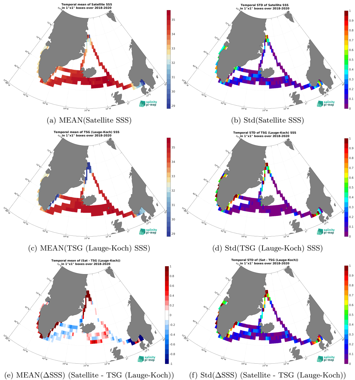
Figure 7: Temporal mean (left) and Std (right) of SSS from SMOS SSS L4 v2 - Daily (BEC) (top), TSG (Lauge-Koch) (middle), and of \Delta SSS (Satellite - TSG (Lauge-Koch)). Only match-up pairs are used to generate these maps.
