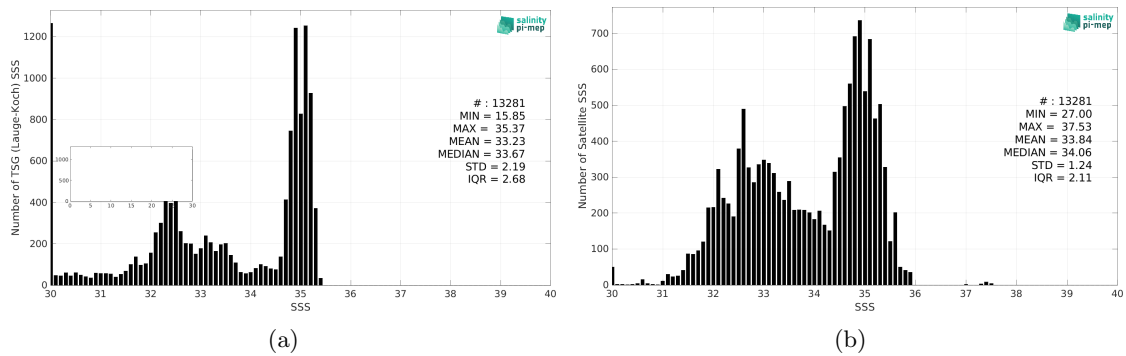
Figure 2: Histograms of SSS from TSG (Lauge-Koch) (a) and SMOS SSS L4 v2 - Daily (BEC) (b) considering all match-up pairs per bins of 0.1 over the Global Ocean Pi-MEP region and for the full satellite product period.
