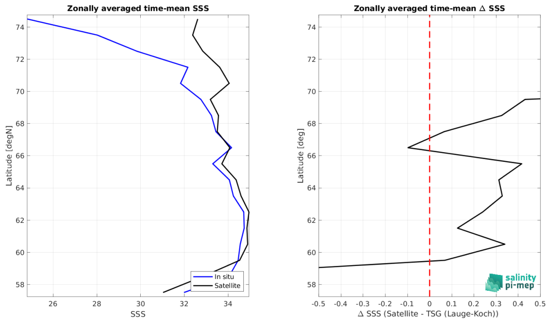
Figure 8: Left panel: Zonal mean SSS from SMOS SSS L4 v2 - Daily (BEC) satellite product (black) and from TSG (Lauge-Koch) (blue). Right panel: Zonal mean of \Delta SSS (Satellite - TSG (Lauge-Koch)) for all the collected Pi-MEP match-up pairs estimated over the full satellite product period.
