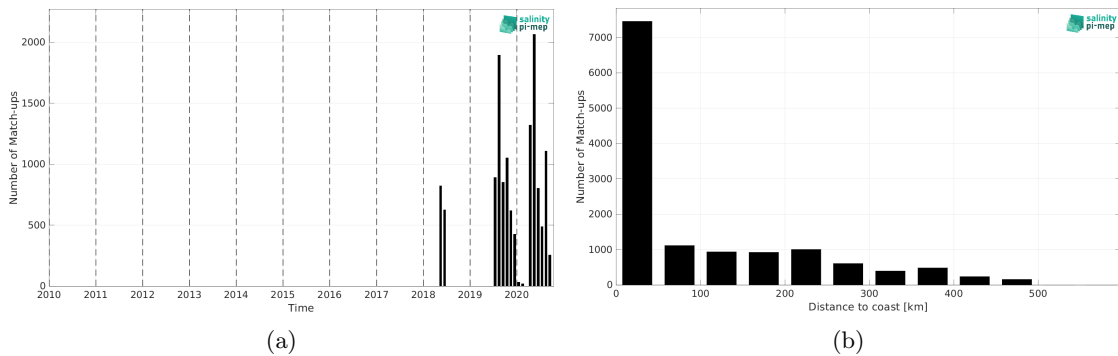
Figure 1: Number of match-ups between TSG (Lauge-Koch) and SMOS SSS L4 v2 - Daily (BEC) SSS as a function of time (a) and as function of the distance to coast (b) over the Global Ocean Pi-MEP region and for the full satellite product period.
