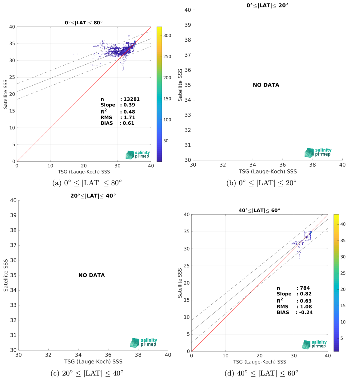
Figure 9: Contour maps of the concentration of SMOS SSS L4 v2 - Daily (BEC) SSS (y-axis) versus TSG (Lauge-Koch) SSS (x-axis) at match-up pairs for different latitude bands. For each plot, the red line shows x=y . The black thin and dashed lines indicate a linear fit through the data cloud and the \pm 95\% confidence levels, respectively. The number match-up pairs n , the slope and R^2 coefficient of the linear fit, the root mean square (RMS) and the mean bias between satellite and in situ data are indicated for each latitude band in each plots.
