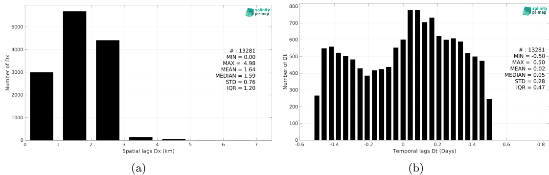
Figure 5: Histograms of the spatial (a) and temporal (b) lags between the location/time of the TSG (Lauge-Koch) measurement and the date of the corresponding SMOS SSS L4 v2 - Daily (BEC) SSS pixel.
