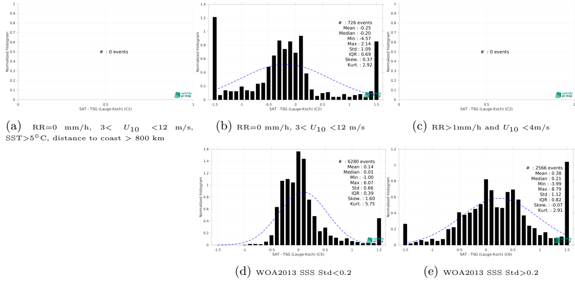
Figure 13: Normalized histogram of \Delta SSS (SMOS SSS L4 v2 - Daily (BEC) - TSG (Lauge-Koch)) for 5 different subdatasets corresponding to: RR=0 mm/h, 3 < U_{10} < 12 m/s, SST > 5°C, distance to coast > 800 km (a), RR=0 mm/h, 3 < U_{10} < 12 m/s (b), RR > 1mm/h and U_{10} < 4 m/s (c), WOA2013 SSS Std < 0.2 (d), WOA2013 SSS Std > 0.2 (e).
