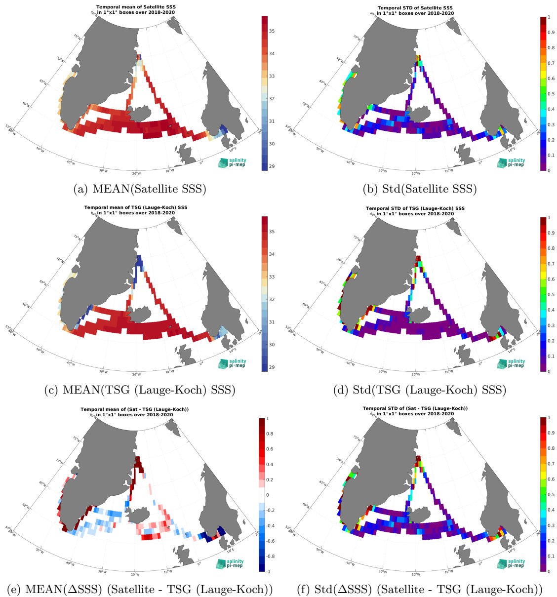
Figure 6: Temporal mean (left) and Std (right) of SSS from SMOS SSS L4 v2 - Daily (BEC) (top), TSG (Lauge-Koch) (middle), and of \Delta SSS (Satellite - TSG (Lauge-Koch)). Only match-up pairs are used to generate these maps.
