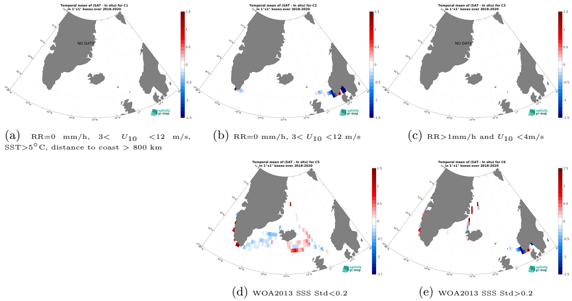
Figure 12: Temporal mean gridded over spatial boxes of size 1^{\circ}\times 1^{\circ} of \Delta\text{SSS} (SMOS SSS L4 v2 - Daily (BEC) - TSG (Lauge-Koch)) for 5 different subdatasets corresponding to:RR=0 mm/h, 3 < U_{10} < 12 m/s, SST >5^{\circ}\text{C} , distance to coast > 800 km (a), RR=0 mm/h, 3 < U_{10} < 12 m/s (b), RR >1 mm/h and U_{10} < 4 m/s (c), WOA2013 SSS Std <0.2 (d), WOA2013 SSS Std >0.2 (e).
