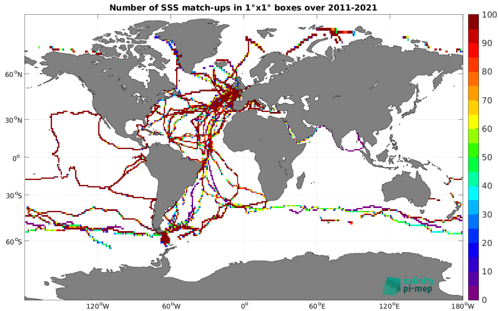
Figure 5: Number of SSS match-ups between TSG (GOSUD-Sailing-ship) SSS and the SMOS SSS L4 v2 - Daily (BEC) SSS product for the Global Ocean Pi-MEP region over 1^\circ \times 1^\circ boxes and for the full satellite product period.
