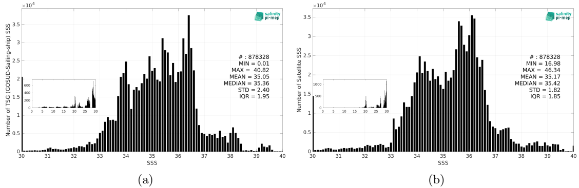
Figure 3: Histograms of SSS from TSG (GOSUD-Sailing-ship) (a) and SMOS SSS L4 v2 - Daily (BEC) (b) considering all match-up pairs per bins of 0.1 over the Global Ocean Pi-MEP region and for the full satellite product period.
