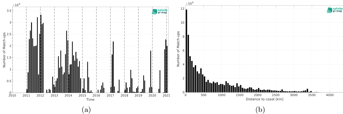
Figure 2: Number of match-ups between TSG (GOSUD-Sailing-ship) and SMOS SSS L4 v2 - Daily (BEC) SSS as a function of time (a) and as function of the distance to coast (b) over the Global Ocean Pi-MEP region and for the full satellite product period.
