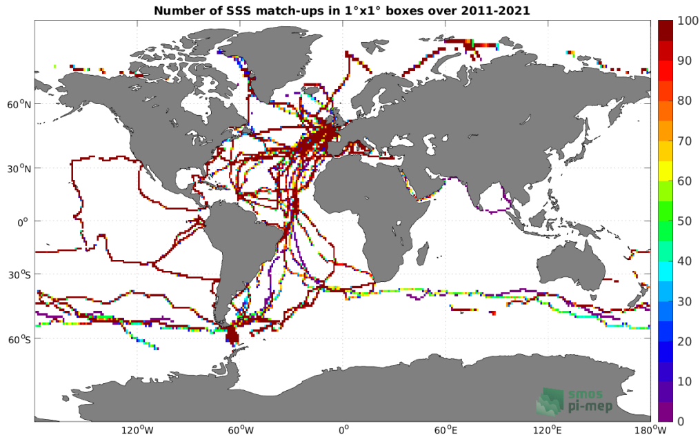
Figure 4: Number of SSS match-ups between TSG (GOSUD-Sailing-ship) SSS and the SMOS SSS L4 v2 - Daily (BEC) SSS product for the Global Ocean Pi-MEP region over 1^\circ \times 1^\circ boxes and for the full satellite product period.
