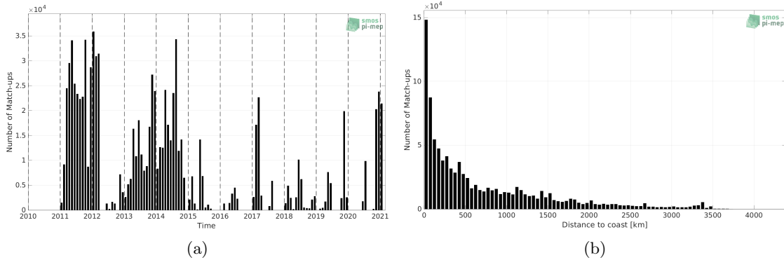
Figure 1: Number of match-ups between TSG (GOSUD-Sailing-ship) and SMOS SSS L4 v2 - Daily (BEC) SSS as a function of time (a) and as function of the distance to coast (b) over the Global Ocean Pi-MEP region and for the full satellite product period.
