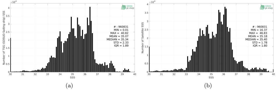
Figure 2: Histograms of SSS from TSG (GOSUD-Sailing-ship) (a) and SMOS SSS L4 v2 - Daily (BEC) (b) considering all match-up pairs per bins of 0.1 over the Global Ocean Pi-MEP region and for the full satellite product period.
