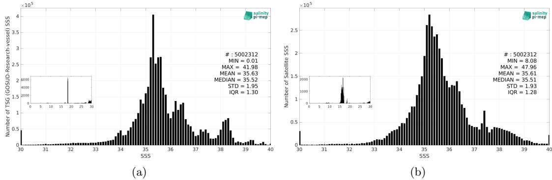
Figure 3: Histograms of SSS from TSG (GOSUD-Research-vessel) (a) and SMOS SSS L4 v2 - Daily (BEC) (b) considering all match-up pairs per bins of 0.1 over the Global Ocean Pi-MEP region and for the full satellite product period.
