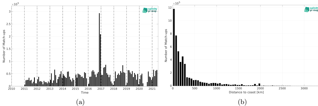
Figure 2: Number of match-ups between TSG (GOSUD-Research-vessel) and SMOS SSS L4 v2 - Daily (BEC) SSS as a function of time (a) and as function of the distance to coast (b) over the Global Ocean Pi-MEP region and for the full satellite product period.
