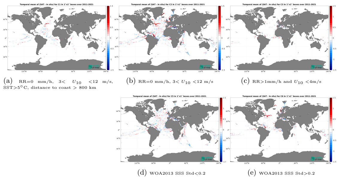
Figure 14: Temporal mean gridded over spatial boxes of size 1^\circ \times 1^\circ of \Delta SSS (SMOS SSS L4 v2 - Daily (BEC) - TSG (GOSUD-Research-vessel)) for 5 different subdatasets corresponding to:RR=0 mm/h, 3 < U_{10} < 12 m/s, SST > 5^\circ\text{C} , distance to coast > 800 km (a), RR=0 mm/h, 3 < U_{10} < 12 m/s (b), RR > 1 mm/h and U_{10} < 4 m/s (c), WOA2013 SSS Std < 0.2 (d), WOA2013 SSS Std > 0.2 (e).
