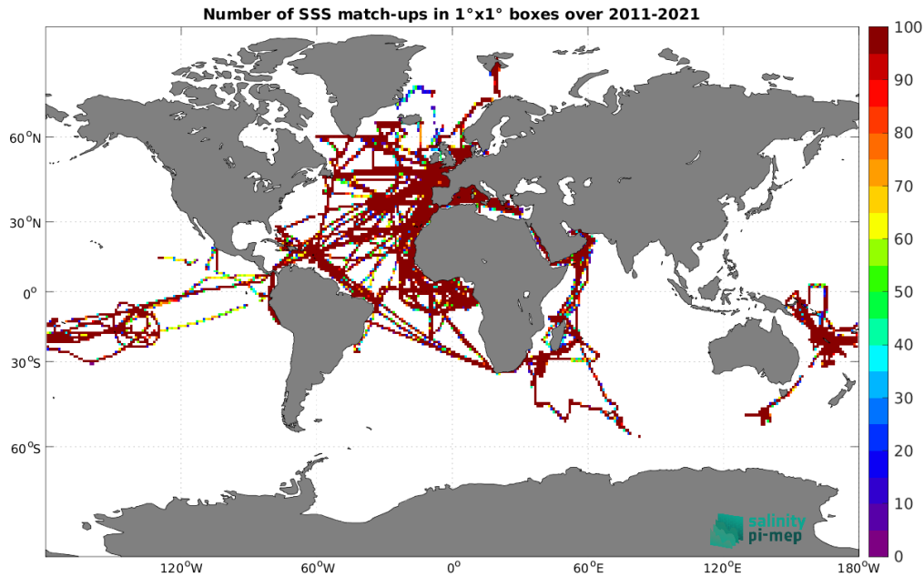
Figure 5: Number of SSS match-ups between TSG (GOSUD-Research-vessel) SSS and the SMOS SSS L4 v2 - Daily (BEC) SSS product for the Global Ocean Pi-MEP region over 1^\circ \times 1^\circ boxes and for the full satellite product period.
