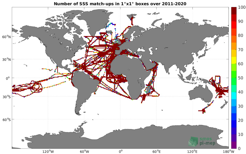
Figure 4: Number of SSS match-ups between TSG (GOSUD-Research-vessel) SSS and the SMOS SSS L4 v2 - Daily (BEC) SSS product for the Global Ocean Pi-MEP region over 1^\circ \times 1^\circ boxes and for the full satellite product period.
