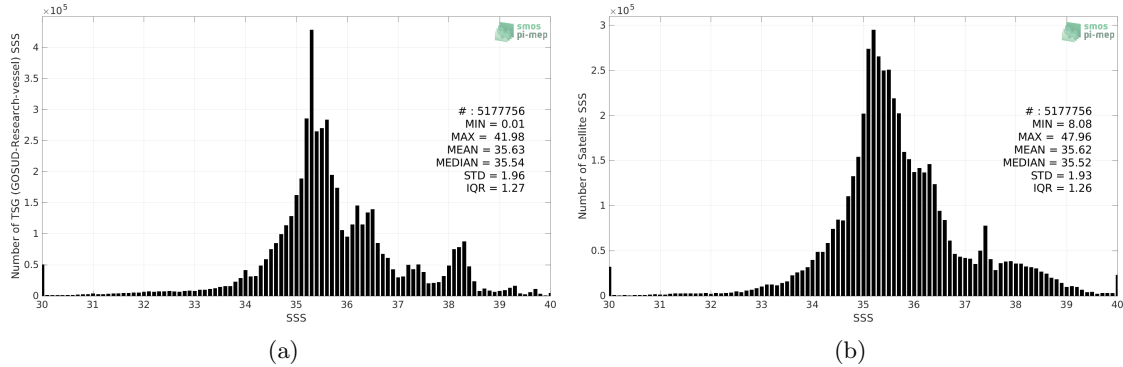
Figure 2: Histograms of SSS from TSG (GOSUD-Research-vessel) (a) and SMOS SSS L4 v2 - Daily (BEC) (b) considering all match-up pairs per bins of 0.1 over the Global Ocean Pi-MEP region and for the full satellite product period.
