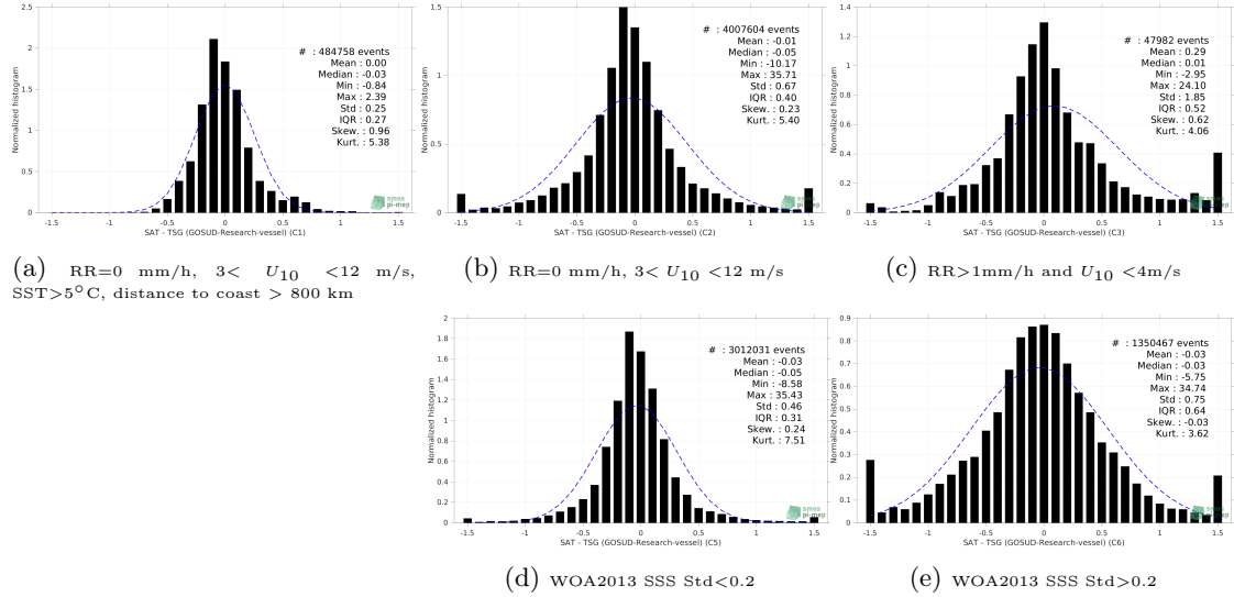
Figure 13: Normalized histogram of \Delta SSS (SMOS SSS L4 v2 - Daily (BEC) - TSG (GOSUD-Research-vessel)) for 5 different subdatasets corresponding to: RR=0 mm/h, 3 < U_{10} < 12 m/s, SST > 5°C, distance to coast > 800 km (a), RR=0 mm/h, 3 < U_{10} < 12 m/s (b), RR > 1mm/h and U_{10} < 4 m/s (c), WOA2013 SSS Std < 0.2 (d), WOA2013 SSS Std > 0.2 (e).
