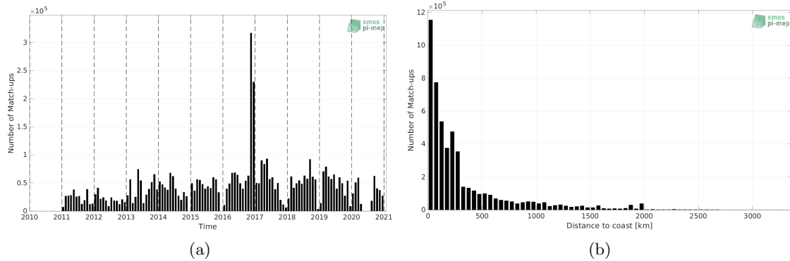
Figure 1: Number of match-ups between TSG (GOSUD-Research-vessel) and SMOS SSS L4 v2 - Daily (BEC) SSS as a function of time (a) and as function of the distance to coast (b) over the Global Ocean Pi-MEP region and for the full satellite product period.
