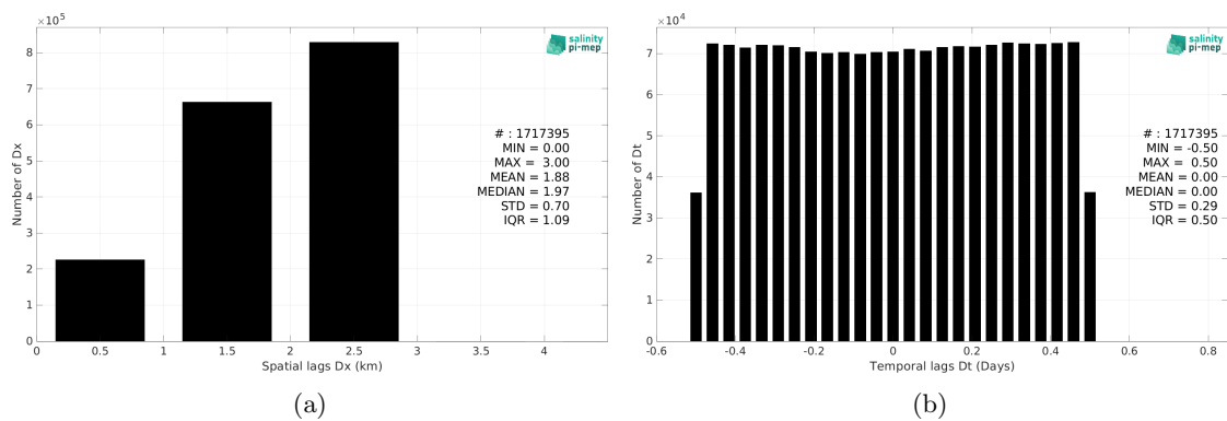
Figure 6: Histograms of the spatial (a) and temporal (b) lags between the location/time of the TSG (CSIC-UTM) measurement and the date of the corresponding SMOS SSS L4 v2 - Daily (BEC) SSS pixel.
