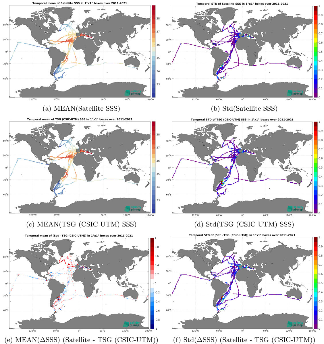
Figure 7: Temporal mean (left) and Std (right) of SSS from SMOS SSS L4 v2 - Daily (BEC) (top), TSG (CSIC-UTM) (middle), and of \Delta SSS (Satellite - TSG (CSIC-UTM)). Only match-up pairs are used to generate these maps.
