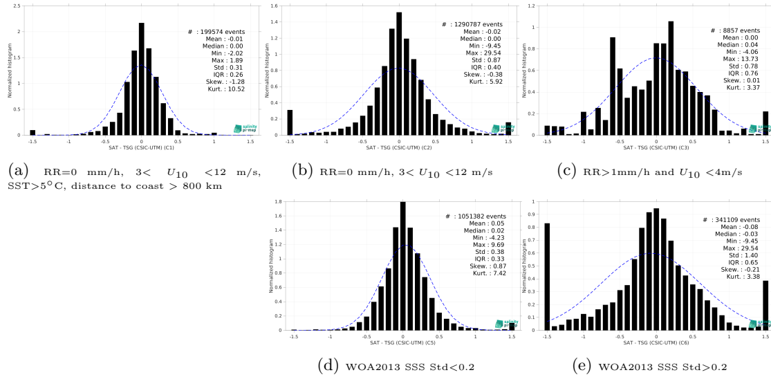
Figure 15: Normalized histogram of \Delta SSS (SMOS SSS L4 v2 - Daily (BEC) - TSG (CSIC-UTM)) for 5 different subdatasets corresponding to: RR=0 mm/h, 3 < U_{10} < 12 m/s, SST>5°C, distance to coast > 800 km (a), RR=0 mm/h, 3 < U_{10} < 12 m/s (b), RR>1mm/h and U_{10} < 4 m/s (c), WOA2013 SSS Std<0.2 (d), WOA2013 SSS Std>0.2 (e).
