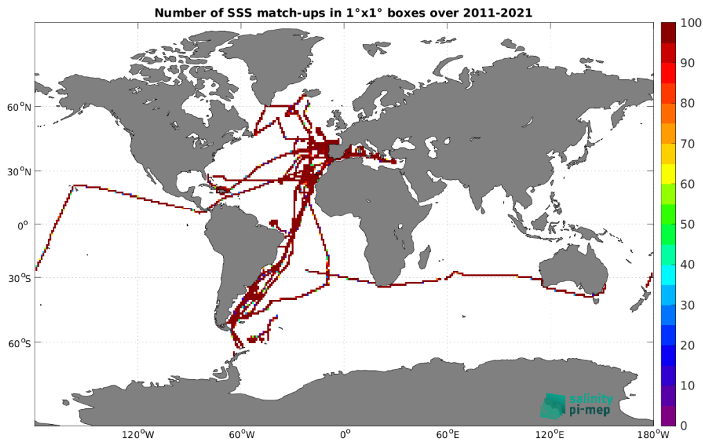
Figure 5: Number of SSS match-ups between TSG (CSIC-UTM) SSS and the SMOS SSS L4 v2 - Daily (BEC) SSS product for the Global Ocean Pi-MEP region over 1^{\circ} \times 1^{\circ} boxes and for the full satellite product period.
