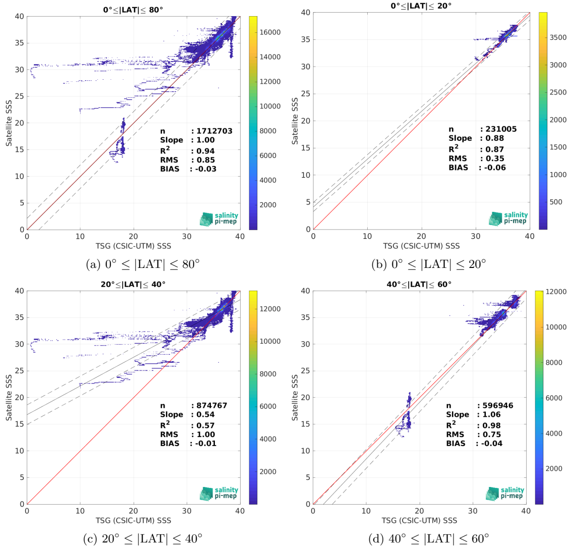
Figure 10: Contour maps of the concentration of SMOS SSS L4 v2 - Daily (BEC) SSS (y-axis) versus TSG (CSIC-UTM) SSS (x-axis) at match-up pairs for different latitude bands. For each plot, the red line shows x=y . The black thin and dashed lines indicate a linear fit through the data cloud and the \pm 95\% confidence levels, respectively. The number match-up pairs n , the slope and R^2 coefficient of the linear fit, the root mean square (RMS) and the mean bias between satellite and in situ data are indicated for each latitude band in each plots.
