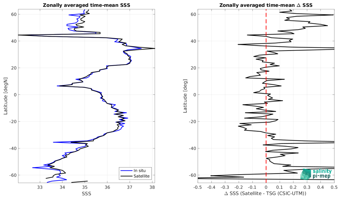
Figure 9: Left panel: Zonal mean SSS from SMOS SSS L4 v2 - Daily (BEC) satellite product (black) and from TSG (CSIC-UTM) (blue). Right panel: Zonal mean of \Delta SSS (Satellite - TSG (CSIC-UTM)) for all the collected Pi-MEP match-up pairs estimated over the full satellite product period.
