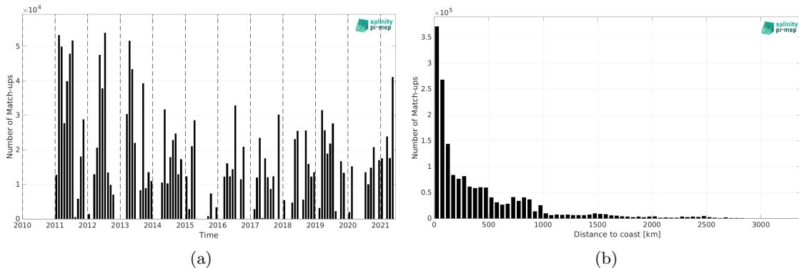
Figure 2: Number of match-ups between TSG (CSIC-UTM) and SMOS SSS L4 v2 - Daily (BEC) SSS as a function of time (a) and as function of the distance to coast (b) over the Global Ocean Pi-MEP region and for the full satellite product period.
