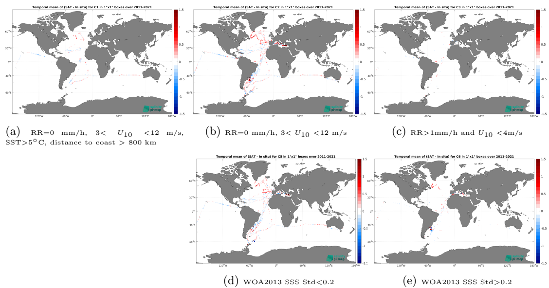
Figure 14: Temporal mean gridded over spatial boxes of size 1^\circ \times 1^\circ of \Delta SSS (SMOS SSS L4 v2 - Daily (BEC) - TSG (CSIC-UTM)) for 5 different subdatasets corresponding to:RR=0 mm/h, 3 < U_{10} < 12 m/s, SST > 5^\circ\text{C} , distance to coast > 800 km (a), RR=0 mm/h, 3 < U_{10} < 12 m/s (b), RR > 1 mm/h and U_{10} < 4 m/s (c), WOA2013 SSS Std < 0.2 (d), WOA2013 SSS Std > 0.2 (e).
