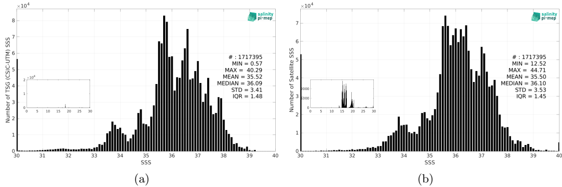
Figure 3: Histograms of SSS from TSG (CSIC-UTM) (a) and SMOS SSS L4 v2 - Daily (BEC) (b) considering all match-up pairs per bins of 0.1 over the Global Ocean Pi-MEP region and for the full satellite product period.
