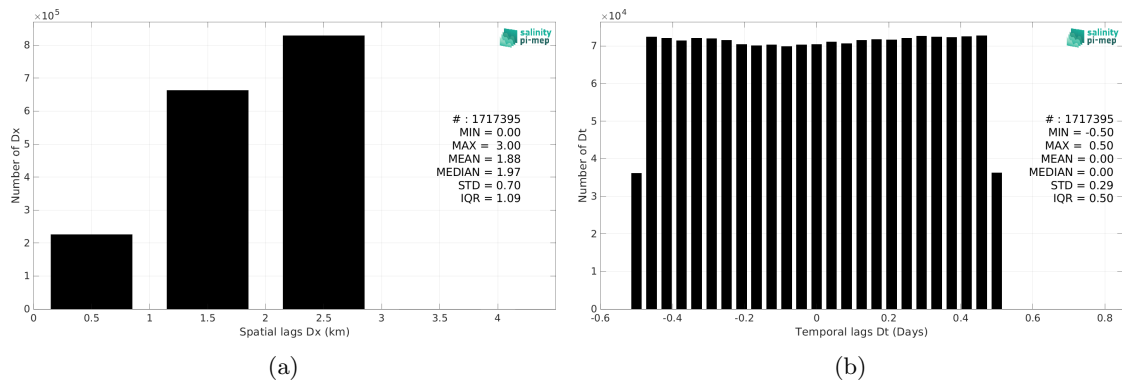
Figure 6: Histograms of the spatial (a) and temporal (b) lags between the location/time of the TSG (CSIC-UTM) measurement and the date of the corresponding SMOS SSS L4 v2 - Daily (BEC) SSS pixel.
